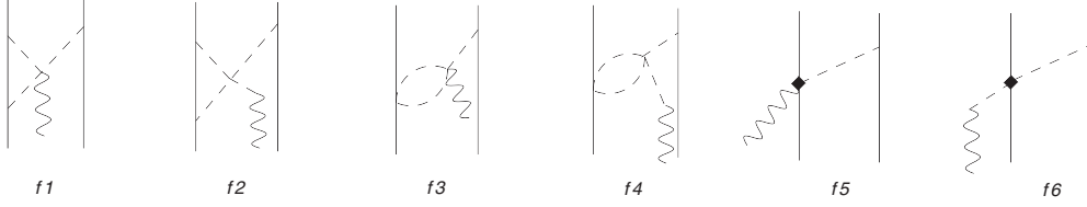
FIG. 10. Additional loop and tree-level corrections of order \mathcal{Q} to the OPE axial charge. Nucleons, pions, and axial fields are denoted by solid, dashed, and wavy lines, respectively. Only a single time ordering is shown for each topology. See text for further explanations.
