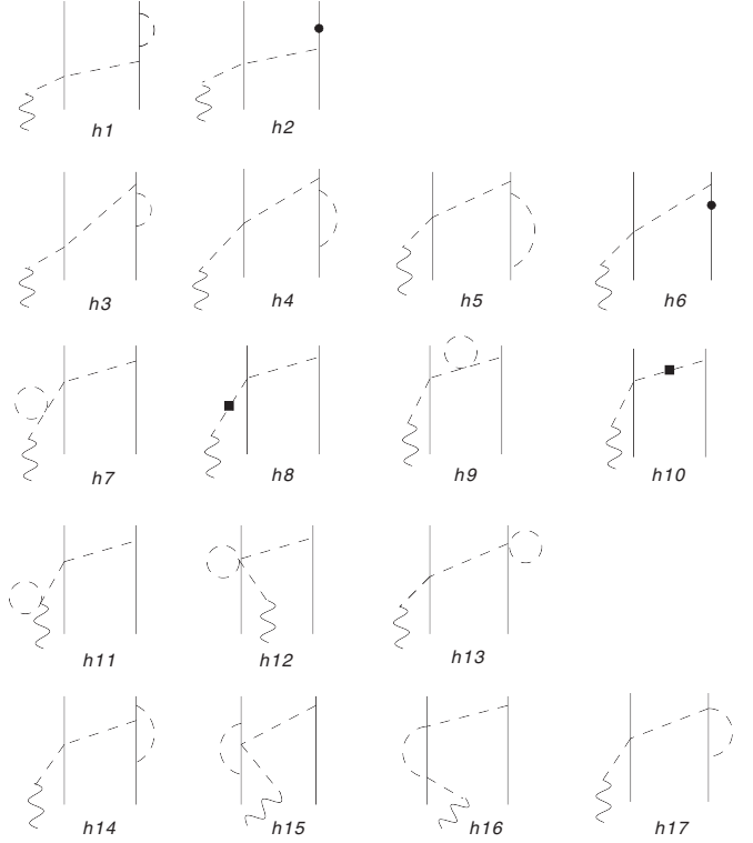
FIG. 9. Representative diagrams for each of the relevant classes contributing to pole corrections to the OPE axial charge at order Q . Nucleons, pions, and axial fields are denoted by solid, dashed, and wavy lines, respectively. More than a single time ordering is shown for some of the diagrams.
