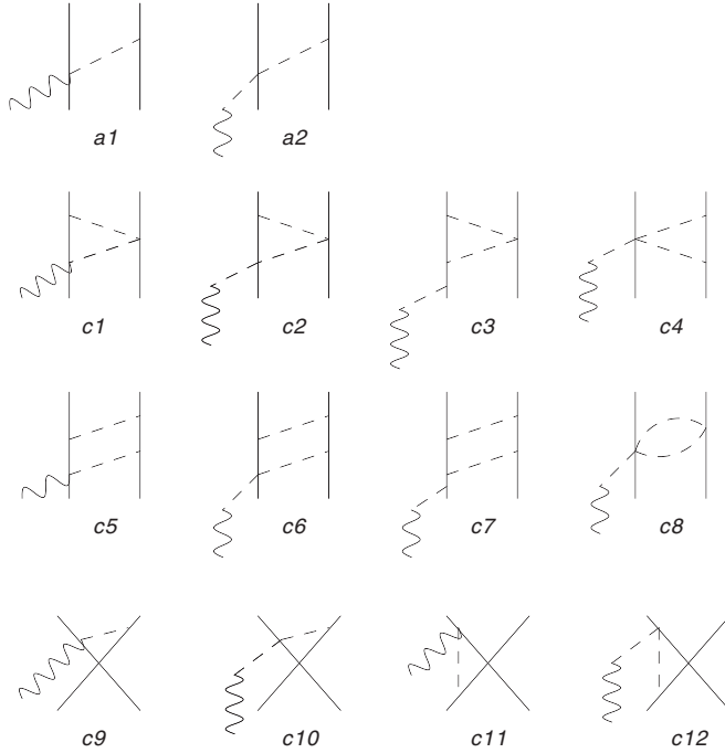
FIG. 2. Diagrams contributing to the OPE axial charge at LO Q^{-1} (panels a1 and a2) and to the TPE axial charge at order Q . Nucleons, pions, and axial fields are denoted by solid, dashed, and wavy lines, respectively. Only a single time ordering is shown for each topology.
