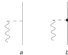
FIG. 13. Feynman amplitudes contributing to the one-body axial charge at LO.
