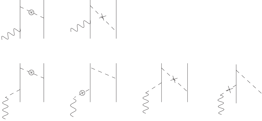
FIG. 12. Illustration of some of the nonstatic corrections to the axial current ignored in this work. Nucleons, pions, and axial fields are denoted by solid, dashed, and wavy lines, respectively. See text for further explanations.
