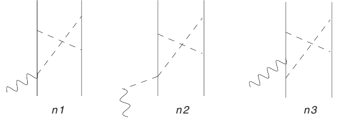
FIG. 14. Diagrams contributing to the axial charge (n1 and n2) and current (n3) at order Q considered in Ref. [18]. Nucleons, pions, and axial fields are denoted by solid, dashed, and wavy lines, respectively. Only a single time ordering is shown for each of the possible 12 (n1) and 60 (n2 and n3) cross-box topologies.
