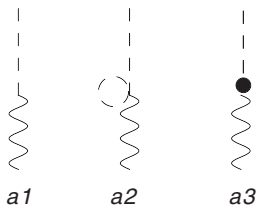
FIG. 5. Diagrams relevant for the renormalization of f_\pi .
