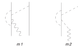
FIG. 11. The only nonvanishing loop corrections to the OPE axial current. Nucleons, pions, and axial fields are denoted by solid, dashed, and wavy lines, respectively. Only a single time ordering is shown for each topology.
