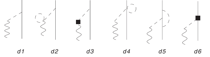
FIG. 7. Pion-pole diagrams.
