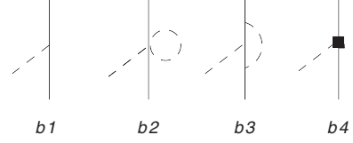
FIG. 6. Diagrams relevant for the renormalization of g_A/f_\pi .
