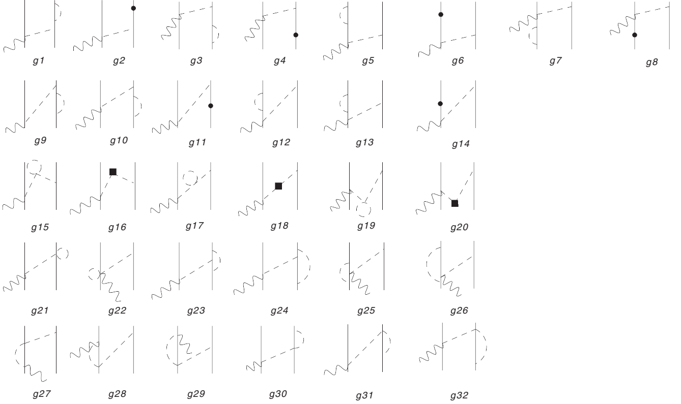
FIG. 8. Half of the possible time-ordered nonpole corrections to the OPE axial charge at order Q . Nucleons, pions, and axial fields are denoted by solid, dashed, and wavy lines, respectively. See text for further explanations.
