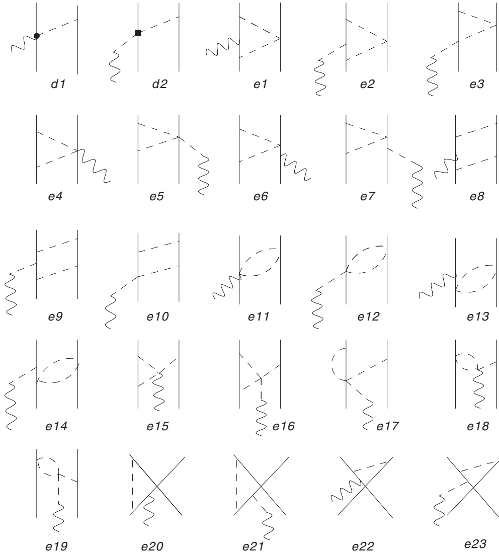
FIG. 4. Diagrams contributing to the OPE axial current at order Q^0 and to the MPE axial current at order Q . Nucleons, pions, and axial fields are denoted by solid, dashed, and wavy lines, respectively. Only a single time ordering is shown for each topology.
