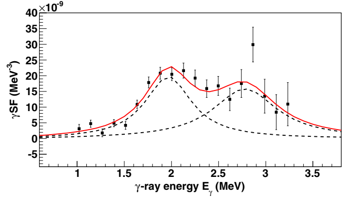
FIG. 5. The extracted \gamma SF for the scissors resonance in the quasicontinuum of ^{243}\text{Pu} .
