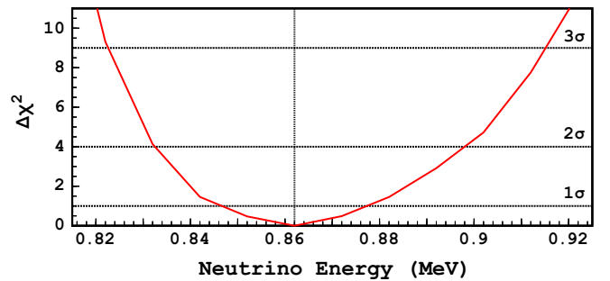
FIG. 6. (Color online) \Delta\chi^2 profile from the fit to the energy of monoenergetic neutrinos discussed in the text. The vertical line indicates the neutrino energy predicted from the ^7\text{Be} electron-capture reaction at 862 keV.
