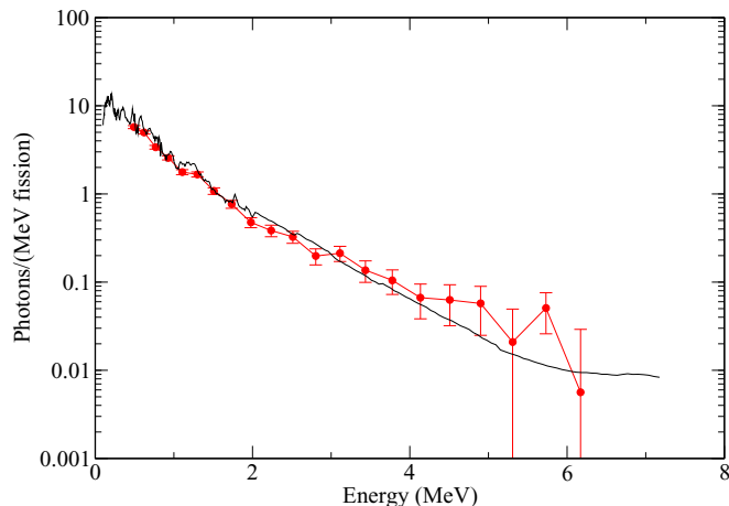
FIG. 3. (Color online) Comparison of PFG emission spectra from fast-neutron-induced fission of ^{235}\text{U} (red circles) from this experiment measured with \text{BaF}_2 detectors with spectra from the thermal-induced fission of ^{235}\text{U} (black line) from a previous experiment [4].
