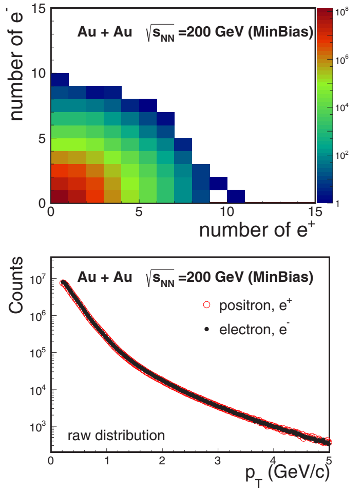
FIG. 4. (Color online) (Top) The distributions of number of electron candidates. (Bottom) Raw p_T spectra of the electron candidates.
