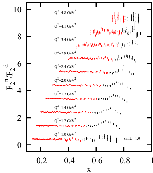
FIG. 1. (Color online) BONuS data for F_2^n/F_2^d vs Bjorken x taken with a 5.26-GeV beam. Only data for Q^2 \geq 1 GeV 2 are shown. The red points ( W > 1.4 GeV) are used in this analysis. Error bars are statistical only. Each spectrum is shifted upward by 1.0 from the set below it.
