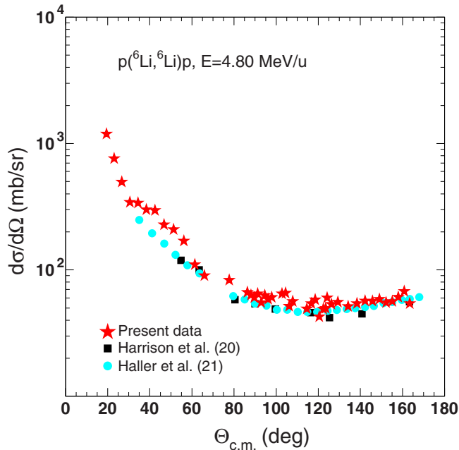
FIG. 6. (Color online) Comparison between present data and previous data ([20,21]) at 4.8 MeV/u.
