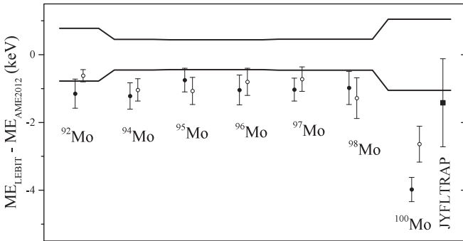
FIG. 5. Comparison of the mass excess values of the LEBIT measurements to AME2012 for ^{92,94-98,100}\text{Mo} with ^{12}\text{C}_8^+ (filled circles) and ^{87}\text{Rb}^+ (open circles) used as reference species. The AME2012 uncertainty for each isotope is shown as the horizontal lines around 0. The JYFLTRAP ^{100}\text{Mo} mass excess comparison is also shown.
