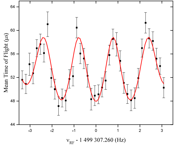
FIG. 2. (Color online) One of 88 ^{96}\text{Zr}^+ time-of-flight Ramsey cyclotron resonances used for the determination of \nu_c(^{96}\text{Zr}^+)/\nu_c(^{96}\text{Mo}^+) . This resonance contains about 1700 detected ^{96}\text{Zr}^+ ions. The solid line is the theoretical line shape [17] fitted to the data.
