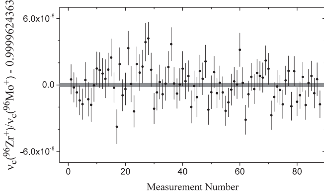
FIG. 3. Data sets of cyclotron frequency ratios v_c(^{96}\text{Zr}^+)/v_c(^{96}\text{Mo}^+) about the set's mean value. The statistical uncertainty in an individual cyclotron frequency ratio is represented by the error bars, and the \pm 1 - \sigma statistical uncertainty of the data set is shown as the shaded band.
