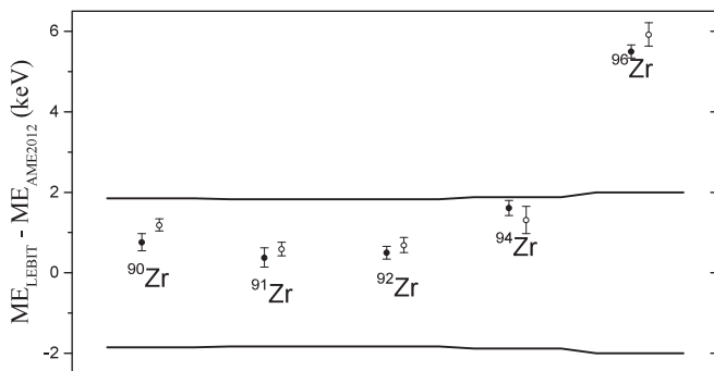
FIG. 4. Comparison of the mass excess values of the LEBIT measurements to AME2012 for ^{90-92,94,96}\text{Zr} with ^{12}\text{C}_8^+ (filled circles) and ^{87}\text{Rb}^+ (open circles) used as reference species. The AME2012 uncertainty for each isotope is shown as the horizontal lines around 0.
