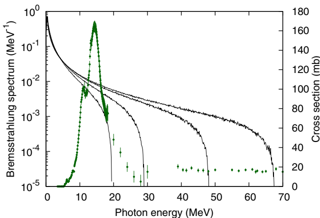
FIG. 3. (Color online) Evaluated cross section of the photofission reaction on ^{238}\text{U} ([42], right axis) and simulated bremsstrahlung spectra at T = 19.5, 29.1, 48.3, 67.7 MeV (left axis) used to calculate the average excitation energies of photofission.
