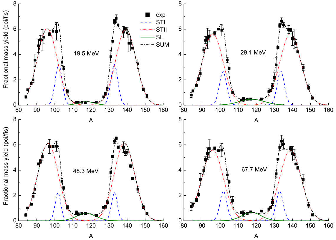
FIG. 4. (Color online) Fraction mass yields ( Y_{\text{FMY}} ) of photofission of ^{238}\text{U} and results of fitting the distributions with five Gaussian curves at bremsstrahlung end-point energies 19.5, 29.1, 48.3, and 67.7 MeV: experimental data (squares), asymmetric component STI (dashed curve), asymmetric component STII (dotted curve), symmetric component SL (solid curve), sum of the components (dashed-dotted curve).
