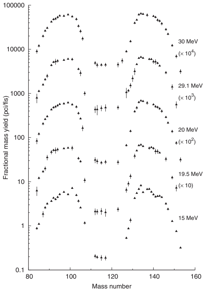
FIG. 5. Comparison of the mass yield distributions of photofission at bremsstrahlung end-point energies T from 15 to 30 MeV. From top to bottom: (1) T = 30 MeV, \langle E^* \rangle = 13.9 MeV (Ref. [21]); (2) T = 29.1 MeV, \langle E^* \rangle = 13.7 MeV (this work); (3) T = 20 MeV, \langle E^* \rangle = 12.9 MeV (Ref. [21]); (4) T = 19.5 MeV, \langle E^* \rangle = 11.9 MeV (this work); (5) T = 15 MeV, \langle E^* \rangle = 10.2 MeV (Ref. [22]).
