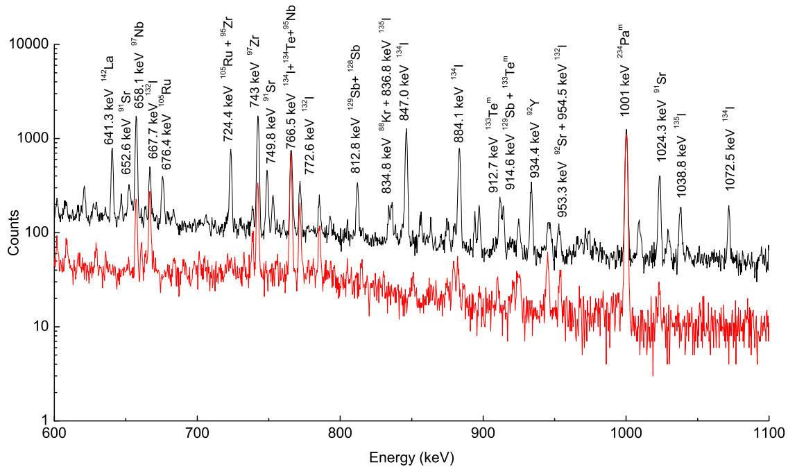
FIG. 1. (Color online) \gamma -ray spectra of induced activity of uranium target after irradiation at T = 29.1 MeV, summed over 10 h. From top to bottom: (1) measurement 1 h after irradiation; (2) measurement 3 days after irradiation.
