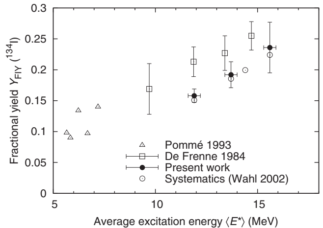
FIG. 2. Relative independent yield of the ^{134}\text{I} isotope as a function of the average excitation energy of ^{238}\text{U} : (dots) present work; Pommé 1993: [36]; De Frenne 1984: [37]; empty dots (Wahl 2002) represent relative independent yield of the ^{134}\text{I} isotope calculated from the systematics [16] for neutron- and proton-induced fission.
