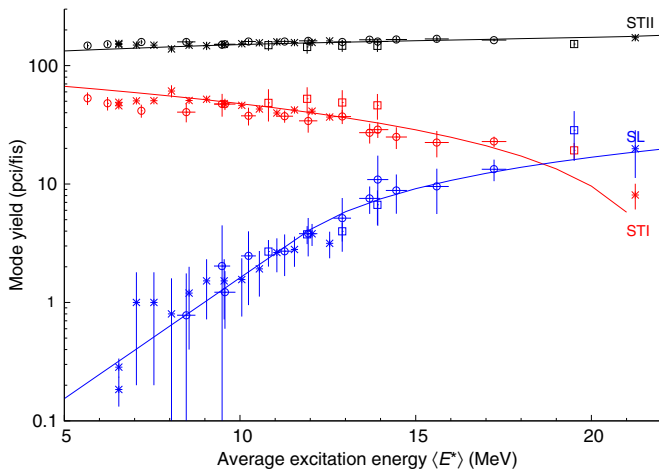
FIG. 7. (Color online) Contributions (weights) of different fission modes in photofission of ^{238}\text{U} and neutron-induced fission of ^{235}\text{U} as a function of the average excitation energy ( E^* ). Circles: contributions of the STII, STI, SL modes of photofission of ^{238}\text{U} calculated from mass distributions obtained in the present work and in works [17,18,20–22]; stars: contributions of the STII, STI, SL modes of neutron-induced fission of ^{235}\text{U} from [15,23,24]; squares: ^{238}\text{U} [24,25]. Mode yields are normalized per 100 fission reactions: Y_{\text{SL}} + Y_{\text{STI}} + Y_{\text{STII}} = 200\% .
