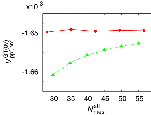
FIG. 2. (Color online) V_{pp',nn'}^{GT(0\nu)}(\bar{E}_a) , an arbitrarily chosen non-negligible one, as a function of effective number of mesh points per dimension N_{\text{mesh}}^{\text{eff}} . [ (N_{\text{mesh}}^{\text{eff}})^2 is equal to the number of mesh points for the (z_1, z_2) plane, and this number is equal to that for the (\rho_1, \rho_2) plane.] This test calculation was performed by using the setup for ^{26}\text{Mg} \rightarrow ^{26}\text{Si} used in Ref. [13] [ \max(z_1) = \max(\rho_1) = 10 \text{ fm} ]. The circles show the result using the scheme shown in Fig. 1, and the triangles show the result using the integral paths from an edge of the square in Fig. 1 to the edge at the opposite side, including the singular points. In the calculations for ^{150}\text{Nd} \rightarrow ^{150}\text{Sm} , it is difficult to use N_{\text{mesh}}^{\text{eff}} \gtrsim 50 because too much memory is required.
