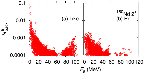
FIG. 7. (Color online) \mathcal{N}_{\text{back}}^a as functions of E_a of (a) the like-particle and (b) proton-neutron QRPA solutions for ^{150}\text{Nd} , (K\pi) = (2+) .
