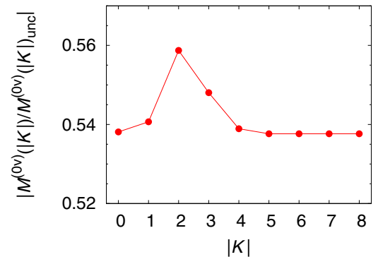
FIG. 6. (Color online) Ratio of |K| component of the NME to that obtained using the HFB state instead of the QRPA ground state in the overlap calculations.
