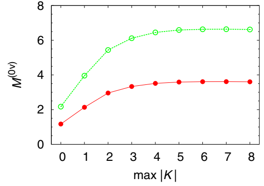
FIG. 5. (Color online) NME obtained by our method (filled circles) and that obtained using the HFB ground states in the calculations of the overlaps (open circles).
