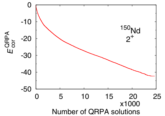
FIG. 4. (Color online) E_{\text{cor}}^{\text{QRPA}} as a function of the number of QRPA solutions for (K\pi) = (2+) , ^{150}\text{Nd} . At each QRPA solution number, the lowest energy solutions are used.
