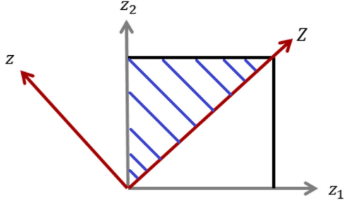
FIG. 1. (Color online) Integral region (inside the square) and integral paths (the lines from z = 0 to the left or top boundary of the square) for calculating the matrix elements of the 0\nu\beta\beta transition operator. The integral with respect to Z is made after the integral with respect to z . The same geometry is applied to a (\rho_1, \rho_2) plane.
