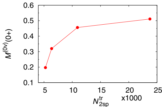
FIG. 3. (Color online) (K\pi) = (0+) component of NME as a function of N_{2\text{sp}}^{\text{tr}} .
