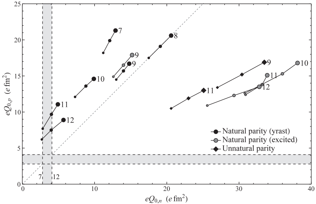
FIG. 18. Intrinsic quadrupole moments plotted as eQ_{0,p} vs eQ_{0,n} for all bands considered in the present work. Bands are distinguished as natural parity yrast (circles, solid), natural parity excited (circles, shaded), and unnatural parity yrast (diamonds). Data points are labeled by the mass number of the Be isotope. Values are shown for successive N_{\max} values ( 6 \leq N_{\max} \leq 10 for natural parity or 7 \leq N_{\max} \leq 11 for unnatural parity) to provide an indication of convergence (the larger symbols indicate higher N_{\max} values) and of the stability of the ratio Q_{0,p}/Q_{0,n} . The line Q_{0,p}/Q_{0,n} = 1 is marked (dashed diagonal line), as is the range of Weisskopf estimates as A ranges from 7 to 12 (shaded bands).
