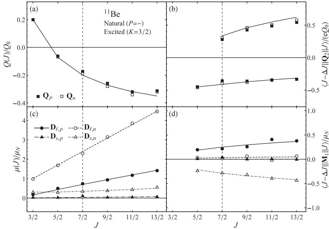
FIG. 10. Dipole and quadrupole matrix element observables for the ^{11}\text{Be} natural parity excited band. See Fig. 5 caption for discussion of the plot contents and labeling.
