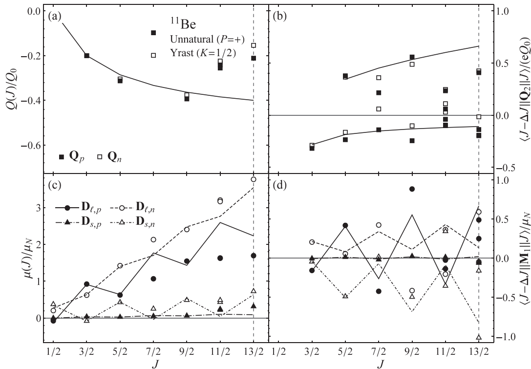
FIG. 11. Dipole and quadrupole matrix element observables for the ^{11}\text{Be} unnatural parity yrast band. See Fig. 5 caption for discussion of the plot contents and labeling.
