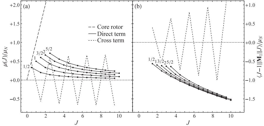
FIG. 2. Rotational predictions for each of the terms contributing, in Eqs. (10) and (11), to (a) magnetic dipole moments and (b) magnetic dipole transition reduced matrix elements, within a rotational band: the core rotor term for dipole moments (dashed line), direct term (solid lines, K \geq 1/2 only, as indicated), and cross term (dotted lines, K = 1/2 only). For purposes of comparison, these terms are shown with equal coefficients, i.e., with a_1 = a_2 = a_3 = \mu_N . Predictions are shown for bands with 0 \leq K \leq 5/2 .
