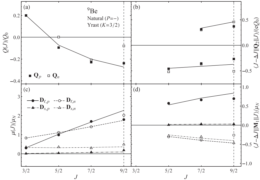
FIG. 6. Dipole and quadrupole matrix element observables for the {}^9\text{Be} natural parity yrast band. See Fig. 5 caption for discussion of the plot contents and labeling.
