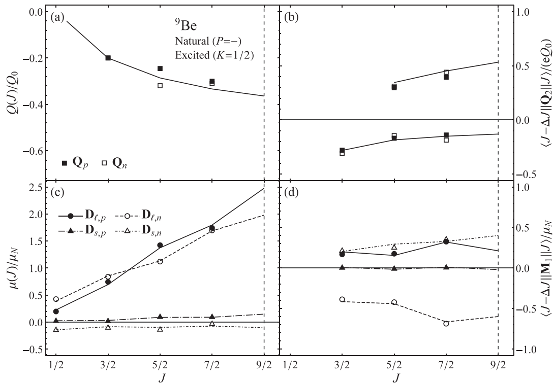
FIG. 7. Dipole and quadrupole matrix element observables for the {}^9\text{Be} natural parity excited band. See Fig. 5 caption for discussion of the plot contents and labeling.
