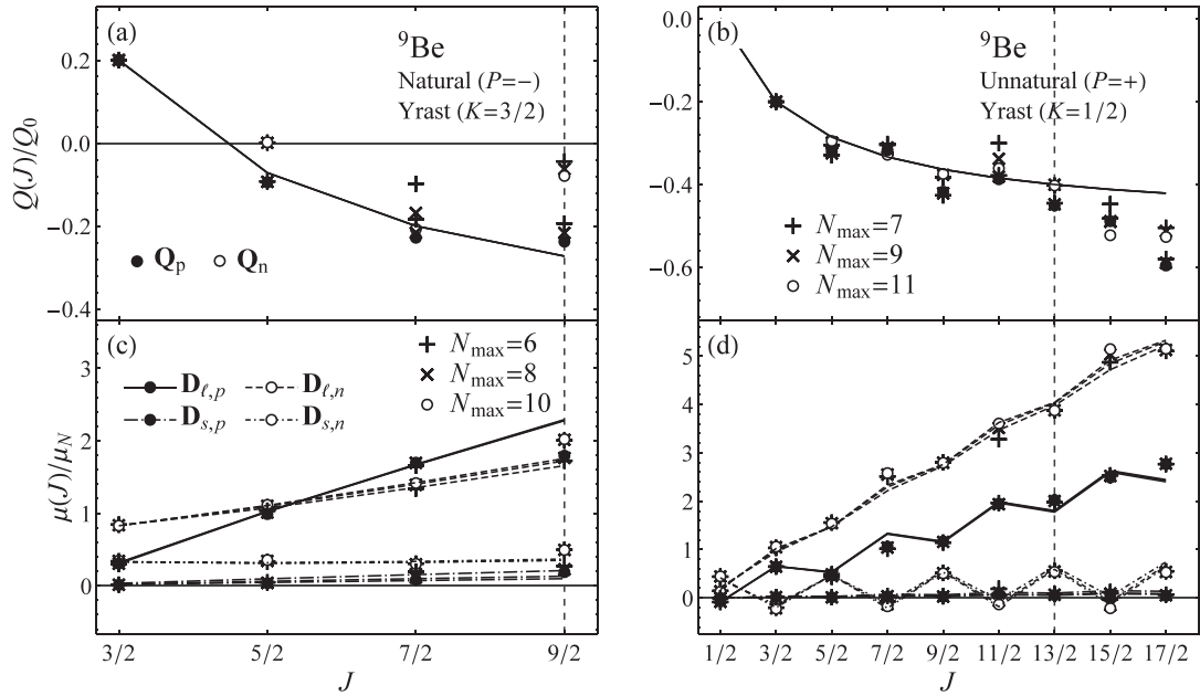
FIG. 17. Dependence of calculated electromagnetic moments for {}^9\text{Be} on the basis truncation N_{\max} : quadrupole moments (top) and dipole moments (bottom) of the natural (left) and unnatural (right) parity yrast bands. Calculations are for 6 \leq N_{\max} \leq 10 for natural parity, or 7 \leq N_{\max} \leq 11 for unnatural parity (calculations of increasing N_{\max} are indicated by pluses, crosses, and circles, respectively). See Fig. 5 caption for discussion of other aspects of the plot contents and labeling.
