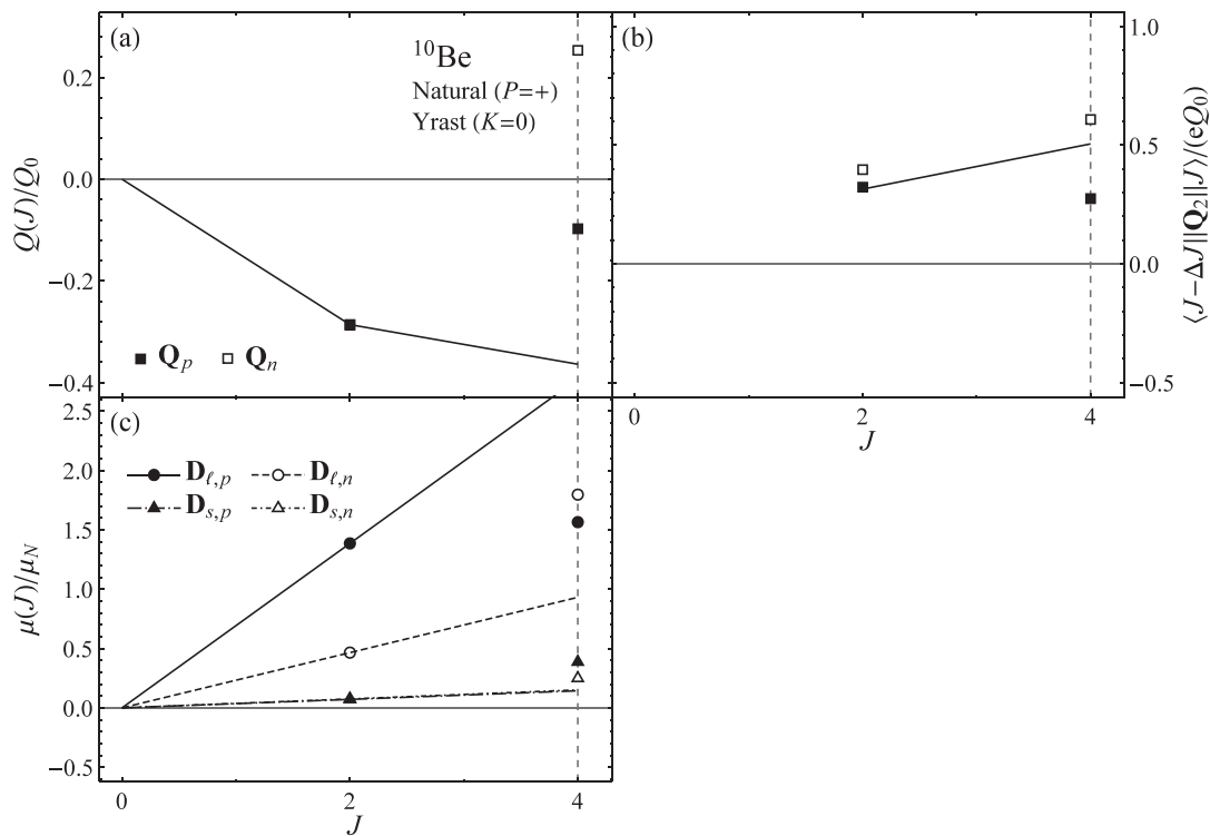
FIG. 13. Dipole and quadrupole matrix element observables for the ^{10}\text{Be} natural parity yrast band. See Fig. 5 caption for discussion of the plot contents and labeling.
