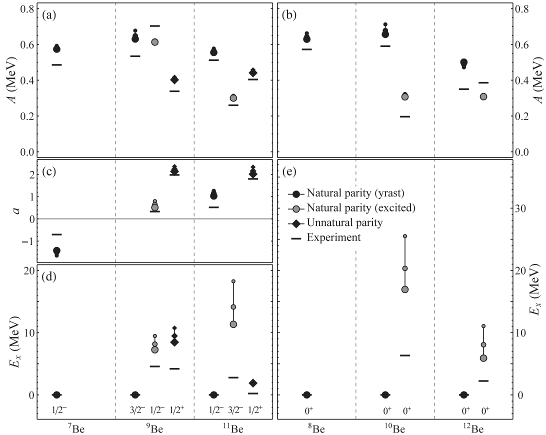
FIG. 19. Band energy parameters for all bands considered in the present work, for the odd-mass Be isotopes (left) and even-mass Be isotopes (right). Parameters considered are the rotational energy constant A (top), the Coriolis decoupling parameter a (middle), and the band excitation energy E_x (bottom), which is defined as the band energy E_0 for the given band [see Eqs. (2) and (3)] relative to that of the natural parity yrast band. Bands are distinguished as natural parity yrast (solid circles), natural parity excited (shaded circles), and unnatural parity yrast (diamonds). Values are shown for successive N_{\max} values ( 6 \leq N_{\max} \leq 10 for natural parity or 7 \leq N_{\max} \leq 11 for unnatural parity) to provide an indication of convergence (the larger symbols indicate higher N_{\max} values). The parameter values extracted from experimental bands are indicated by horizontal lines. The K^P assignments for the bands are indicated at bottom.
