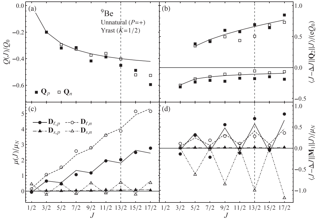
FIG. 8. Dipole and quadrupole matrix element observables for the {}^9\text{Be} unnatural parity yrast band. See Fig. 5 caption for discussion of the plot contents and labeling.
