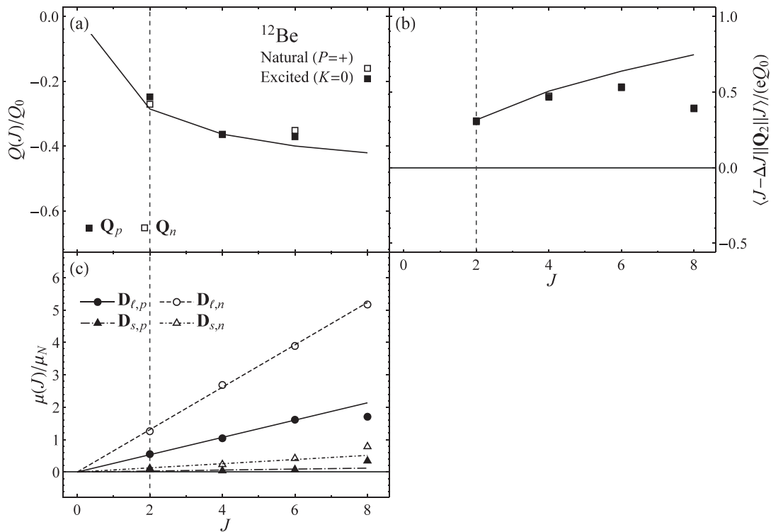
FIG. 15. Dipole and quadrupole matrix element observables for the ^{12}\text{Be} natural parity excited band. See Fig. 5 caption for discussion of the plot contents and labeling.
