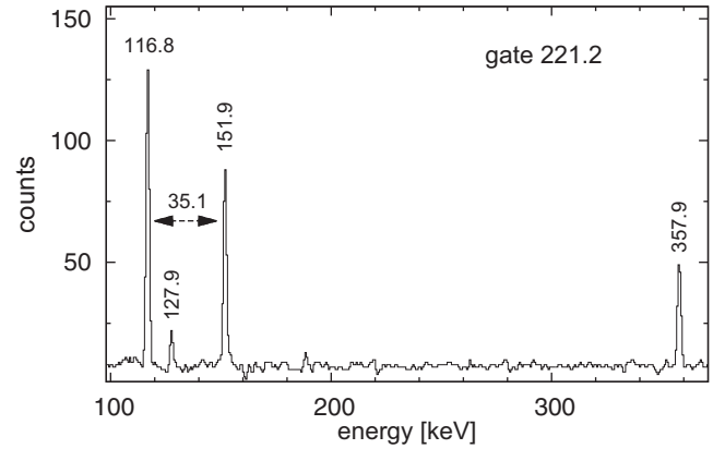
FIG. 12. A spectrum of \gamma rays following \beta^- decay of ^{113}\text{Rh} measured in the mass A = 113 separated with the IGISOL facility. The gate is set on the 221.2-keV line. Peaks are labeled with their energies in keV.
