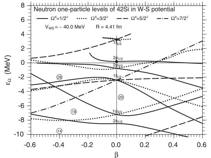
FIG. 1. Calculated one-particle energies for neutrons of ^{42}_{14}\text{Si}_{28} as a function of axially symmetric quadrupole deformation. Bound one-particle energies at \beta = 0 are -8.50 , -7.24 , -2.42 , and -0.77 MeV for the 2s_{1/2} , 1d_{3/2} , 1f_{7/2} , and 2p_{3/2} levels, respectively, while one-particle resonant 2p_{1/2} and 1f_{5/2} levels are obtained at +0.20 MeV with the width of 0.20 MeV and +3.25 MeV with the width of 0.58 MeV, respectively, which are denoted by filled circles. The resonant \Omega^\pi = 1/2^- level which is connected to the resonant 2p_{1/2} level at \beta = 0 cannot be obtained for \beta < -0.19 corresponding to \varepsilon_\Omega > 1.42 MeV. One-particle resonant energies for \beta \neq 0 are not plotted unless they are important for the present discussion. For simplicity, calculated widths of one-particle resonant levels are not shown. The neutron numbers, 14, 18, 20, and 28, which are obtained by filling all lower-lying levels, are indicated with circles. One-particle levels with \Omega = 1/2, 3/2, 5/2 , and 7/2 are expressed by solid, dotted, long-dashed, and dot-dashed curves, respectively, for both positive and negative parities. The parity of levels can be seen from the \ell values denoted at \beta = 0 ; \pi = (-1)^\ell .
