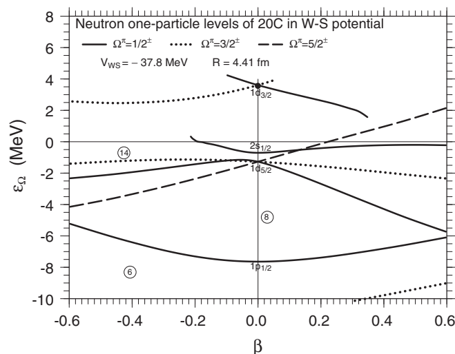
FIG. 2. Calculated one-particle energies for neutrons of {}^{20}\text{C}_{14} as a function of axially symmetric quadrupole deformation. Bound one-particle energies at \beta = 0 are -7.66 , -1.28 , and -0.71 MeV for the 1p_{1/2} , 1d_{5/2} , and 2s_{1/2} levels, respectively, while one-particle resonant 1d_{3/2} level is obtained at +3.57 MeV with the width of 3.02 MeV. The resonant \Omega^\pi = 1/2^+ level which is connected to the bound 2s_{1/2} level at \beta = 0 cannot be obtained for \beta < -0.215 corresponding to \varepsilon_\Omega > 0.38 MeV. On the other hand, the resonant \Omega^\pi = 1/2^+ level connected to the resonant 1d_{3/2} level at \beta = 0 cannot be obtained for \beta > 0.35 corresponding to \varepsilon < 1.54 MeV, because in the deformation region the s_{1/2} component becomes appreciable in the wave function. For smaller \beta values the major component of the wave function of the \Omega^\pi = 1/2^+ level is 1d_{3/2} and, thus, the resonant level survives. The neutron numbers, 6, 8, and 14, which are obtained by filling all lower-lying levels, are indicated with circles. One-particle levels with \Omega = 1/2 , 3/2 , and 5/2 are expressed by solid, dotted, and long-dashed curves, respectively, for both positive and negative parities.
