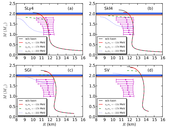
FIG. 3. (Color online) Mass-radius curve for each of the four SkH models. Thick blue and thick orange solid straight lines are recent observations [6,7]. Filled circles with error bars denote the allowed mass and radius ranges obtained from the analysis by Steiner et al. [16].
