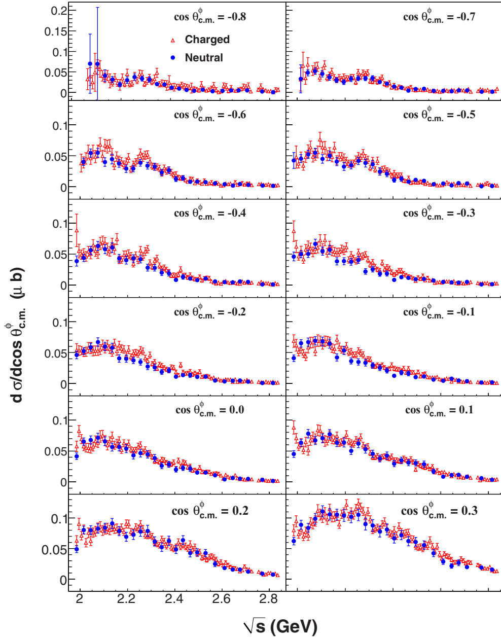
FIG. 16. (Color online) Comparison of the charged- and neutral-mode d\sigma/d\cos\theta_{c.m.}^\phi results in 0.1- \cos\theta_{c.m.}^\phi bins, at mid and backward angles. The charged-mode results comprise the two-track data set with additional \Lambda^* cuts as explained in the text. The y-axis range is constant over each horizontal row and is shown in the left-most column for every row. All error bars represent statistical uncertainties only.
