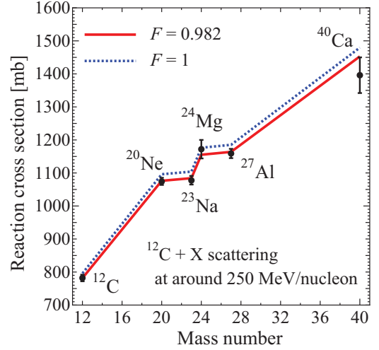
FIG. 1. (Color online) Reaction cross sections for the ^{12}\text{C} scattering on stable nuclei from A = 12 to 40 . The data for ^{12}\text{C} and ^{27}\text{Al} at 250.8 MeV/nucleon are taken from Ref. [48]. The data for ^{20}\text{Ne} and ^{23}\text{Na} at 250 MeV/nucleon are deduced from the measured \sigma_1 at around 1 GeV/nucleon [49,50] with the Glauber model [17]. The data for ^{40}\text{Ca} at 240 MeV/nucleon is obtained from the measured \sigma_R at 83 MeV/nucleon [51] with the Glauber model [18]. The solid (dotted) line stands for the results of the folding-model calculations after (before) the normalization with a factor F = 0.982 .
