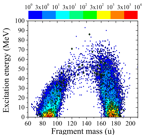
FIG. 5. (Color online) Excitation energy of primary fragments formed in the reaction ^{88}\text{Sr}+^{176}\text{Yb} at E_{\text{c.m.}} = 290 MeV.
