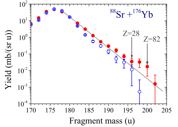
FIG. 4. (Color online) Double differential cross sections of heavy fragments formed in the reaction ^{88}\text{Sr}+^{176}\text{Yb} at E_{\text{c.m.}} = 290 MeV and detected at laboratory angles from 25^\circ up to 35^\circ . Filled circles indicate the primary mass distribution, and open circles indicate the mass distribution corrected for neutron emission.
