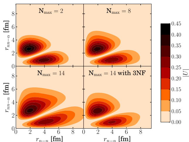
FIG. 3. (Color online) Model-space dependence of the three-body channel form factor ( {}^6\text{He}(0^+)|{}^4\text{He}(0^+) + n + n ). The main L = S = 0 channel is shown for a sequence of calculations with increasing N_{\text{max}} performed with \Lambda_{\text{SRG}} = 2.0 \text{ fm}^{-1} and \hbar\Omega = 16 \text{ MeV} . The lower right panel shows the same contour plot using an SRG-evolved chiral NN + 3NF interaction [43].
