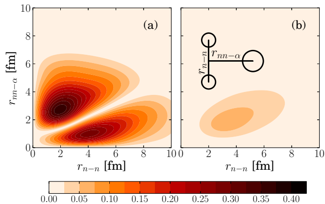
FIG. 2. (Color online) Contour plots of the translationally invariant three-body channel form factor ( {}^6\text{He}(0^+)|{}^4\text{He}(0^+) + n + n ) calculated from NCSM wave functions. The two allowed channels for this overlap, L = S = 0 and L = S = 1 , are shown in panels (a) and (b), respectively.
