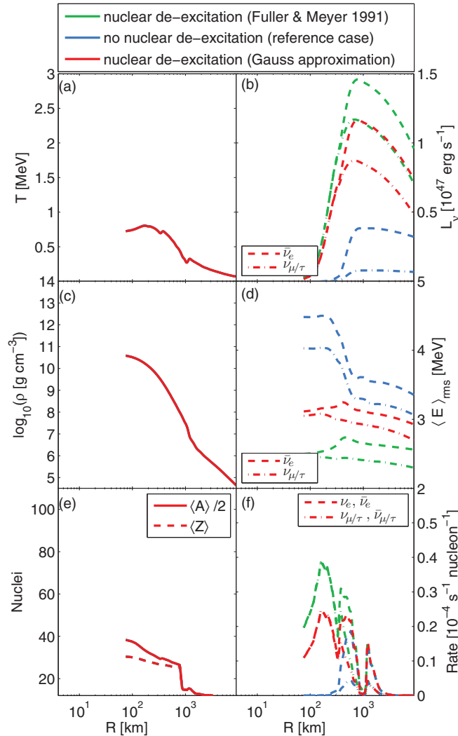
FIG. 5. (Color online) Radial profile of selected quantities at about 50 ms before core bounce, comparing simulations for which we include the production of neutrino pairs from heavy-nuclei de-excitations, based on Ref. [8] (green lines), and the Gauss approximation expression (26) (red lines), in comparison to a simulation that uses the standard set of weak rates as listed in Table I (blue lines) and otherwise identical input physics.
