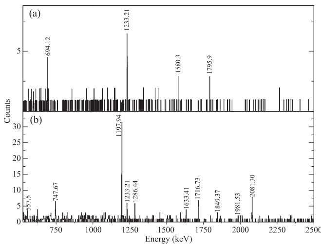
FIG. 10. (a) The \gamma rays between 525 and 2500 keV in coincidence with (a) the 53-keV 0_1^+ \rightarrow 2_1^+ and 509-keV 0_1^+ \rightarrow 0_{\text{gs}}^+ conversion-electron transitions and (b) the \gamma rays in coincidence with the 456-keV 2_1^+ \rightarrow 0_{\text{gs}}^+ \gamma ray following the \beta decay of ^{74}\text{Rb} .
