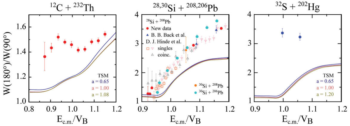
FIG. 5. (Color online) Observed and calculated anisotropies are shown for reactions using the lightest three projectiles. The angular anisotropy data presented for ^{12}\text{C} + ^{232}\text{Th} are from Ref. [37]; data presented for ^{28}\text{Si} + ^{208}\text{Pb} have been taken from Refs. [53,57]. All other data are from this work. The TSM calculation results (presented as solid lines) are shown for calculations using three different diffuseness parameters, as discussed in Sec. IV. For the middle panel, TSM calculations are for ^{30}\text{Si} + ^{206}\text{Pb} , using the same color scheme for the diffuseness parameters as shown in the legend for the panel to the right. In all three cases, the TSM is inconsistent with experiment.
