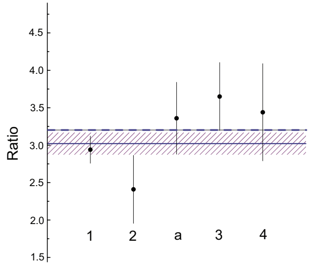
FIG. 4. (Color online) Ratio between experimental cross sections for excitation of ^{13}\text{Be} resonances obtained in ^1\text{H}(^{14}\text{Be}, ^{12}\text{Be} + n) at 69 MeV/nucleon and 304 MeV/nucleon. The obtained ratio 3.0(1) is close to the one given in Ref. [51] shown as the dashed line. The labeling of the resonances is the same as in Fig. 3.
