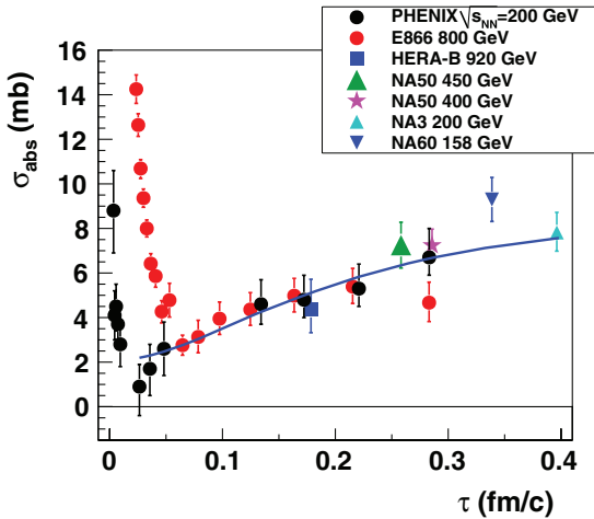
FIG. 8. (Color online) The same data as in Fig. 7 plotted on a linear scale compared to a calculation of the cross section based on the model of Ref. [22].
