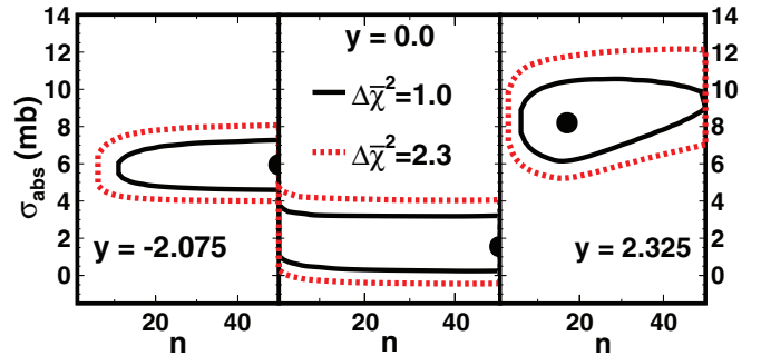
FIG. 2. (Color online) The \bar{\chi}^2 distributions for the most backward, mid- and most forward rapidities when \sigma_{\text{abs}} and n are optimized separately at each rapidity.
