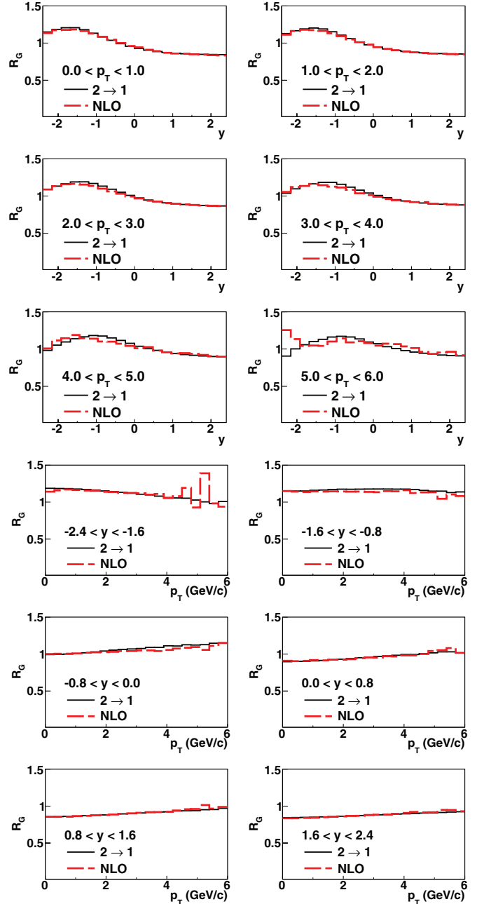
FIG. 1. (Color online) Comparison of the gluon modification as a function of rapidity and p_T obtained from EPS09 NLO using x and Q^2 values from Eq. (1) and from the CEM calculation [15], NLO in the total cross section.
