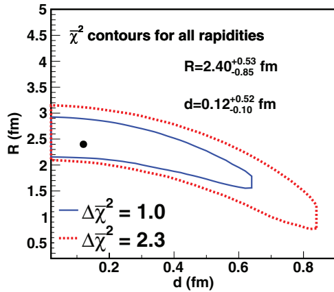
FIG. 4. (Color online) The \bar{\chi}^2 contours obtained from the fits with global values of R and d , Eq. (6). The uncertainties in R and d are taken from the maximum extent of the \Delta\bar{\chi}^2 = 1 contour.
