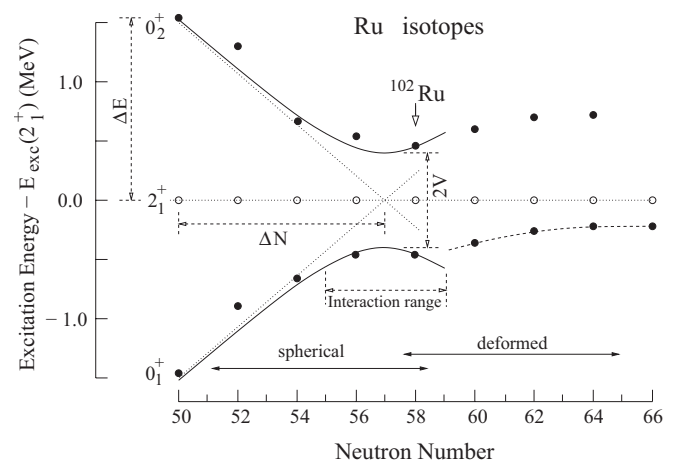
FIG. 4. Positions of 0_1^+ and 0_2^+ levels (full dots), relative to the 2_1^+ phonon excitation (open dots) in Ru isotopes. Solid lines represent a two-level mixing calculation. Symbols shown in the figure are explained in the text.
