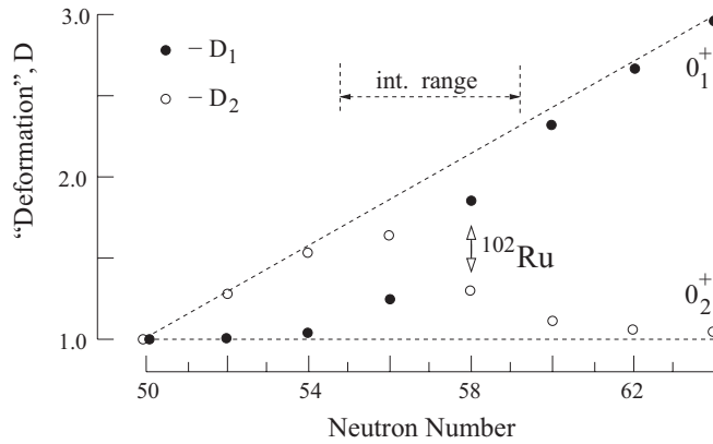
FIG. 5. Exchange of properties between the crossing 0_1^+ and 0_2^+ levels, as simulated in two-level mixing calculation. See text for the explanation of D_1 and D_2 and further comments.
