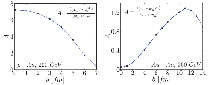
FIG. 1. (Color online) Asymmetry in wounded nucleons in p + Au (left) and Au + Au (right) collisions at \sqrt{s} = 200 GeV as a function of the impact parameter b .
