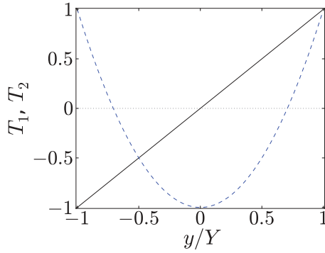
FIG. 2. (Color online) Two components of the fluctuating fireball rapidity density: An asymmetry (solid black line) and a butterfly (dashed blue line).
