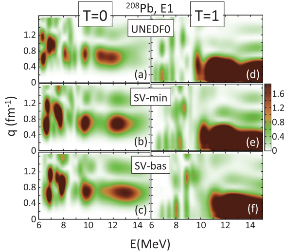
FIG. 3. (Color online) Similar to Fig. 2, for (a–c) T = 0 and (d–f) T = 1 E1 strength computed with (a) UNEDF0, (b) SV-min, and (c) SV-bas EDFs.
