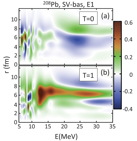
FIG. 4. (Color online) Energy-averaged E1 transition density in ^{208}\text{Pb} calculated with SV-bas as a function of E and r for (a) T = 0 and (b) T = 1 .
