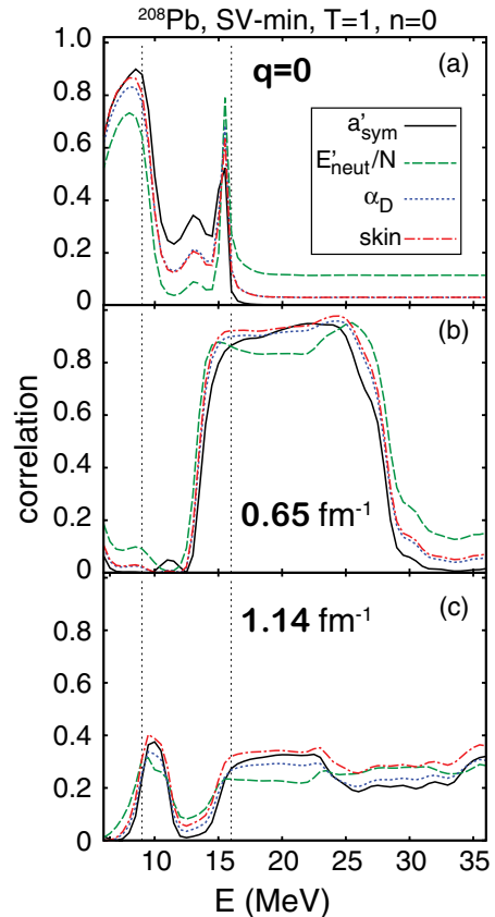
FIG. 9. (Color online) Correlation between the T = 1 accumulated E1 strength in ^{208}\text{Pb} and selected isovector indicators ( a'_{\text{sym}} , E'_{\text{neut}}/N , \alpha_D , r_{\text{skin}} ) in SV-min as a function of E for (a) q = 0 , (b) q = 0.65 \text{ fm}^{-1} , and (c) q = 1.14 \text{ fm}^{-1} .
