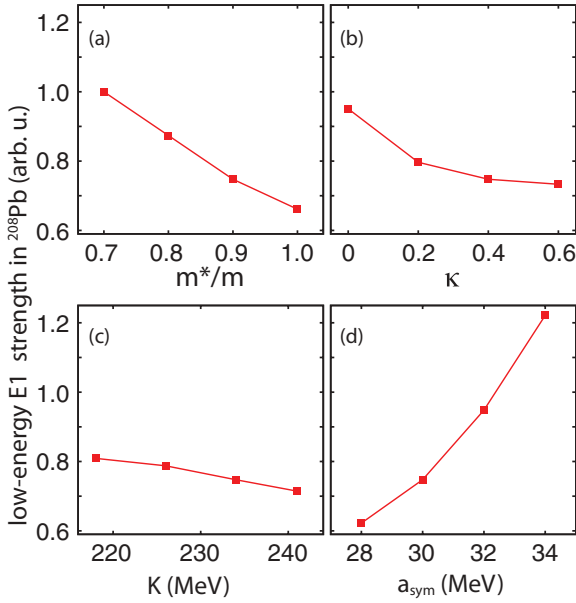
FIG. 5. (Color online) Dependence of the low-energy E1 strength, (7), in ^{208}\text{Pb} on selected NMP: (a) m^*/m , (b) \kappa , (c) K , and (d) a_{\text{sym}} . Calculations were carried out with the SV-bas family of EDFs. The cutoff energy is E_{\text{max}} = 10 MeV.
