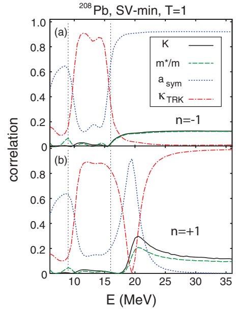
FIG. 6. (Color online) Correlation between the energy-weighted accumulated strength A_n^D(E) , (5), in ^{208}\text{Pb} and selected NMP (incompressibility K , isoscalar effective mass m^*/m , symmetry energy a_{\text{sym}} , and TRK sum rule enhancement \kappa ) as a function of E obtained with SV-min. (a) n = -1 ; (b) n = 1 . The GDR region is marked by vertical dotted lines.
