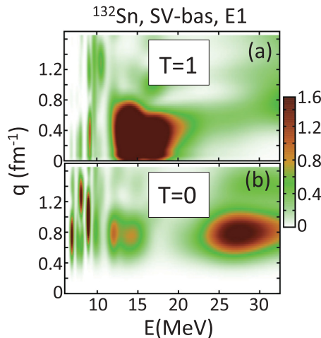
FIG. 11. (Color online) Similar to Figs. 2(c) and 2(d), except for ^{132}\text{Sn} .
