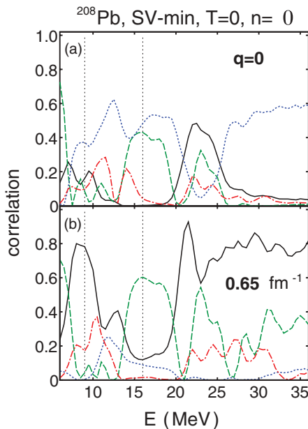
FIG. 8. (Color online) Similar to Fig. 7, but for the T = 0 compressional dipole E1 strength.
