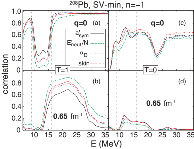
FIG. 10. (Color online) Correlation between (a, b) the T = 1 and (c, d) the T = 0 accumulated inverse-energy-weighted E1 strength A_{-1}^F in ^{208}\text{Pb} and selected isovector indicators ( a'_{\text{sym}} , E'_{\text{neut}}/N , \alpha_D , r_{\text{skin}} ) in SV-min as a function of E for (a, c) q = 0 and (b, d) q = 0.65 \text{ fm}^{-1} .
