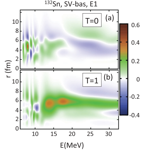
FIG. 12. (Color online) Similar to Fig. 4, except for ^{132}\text{Sn} .
