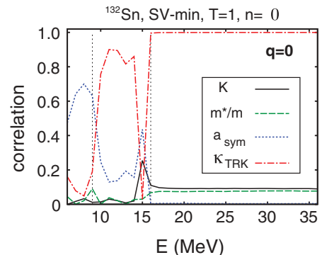
FIG. 13. (Color online) Similar to Fig. 7(a), except for ^{132}\text{Sn} .
