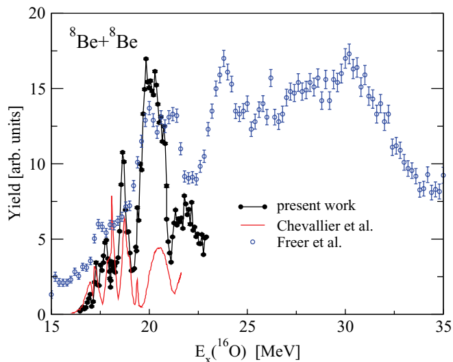
FIG. 5. (Color online) ^{16}\text{O} excitation energy spectra for the ^8\text{Be} + ^8\text{Be} decay channel. The data from the ^{12}\text{C}(^4\text{He}, ^8\text{Be})^8\text{Be} reaction from the present measurements and those of Chevallier et al. [3] are compared with the spectrum for the ^{12}\text{C}(^{12}\text{C}, ^8\text{Be} + ^8\text{Be})^8\text{Be} measured at a beam energy of 84 MeV [7].
