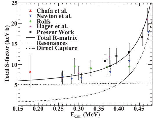
FIG. 10. (Color online) Comparison of the S factor obtained from the R -matrix fit of the present data set with literature experimental data. The thick continuous line represents the extrapolation of the total S factor from the best R -matrix fit, with background poles included and some ANC values fixed (“Total R -matrix”). The dashed-dotted line and the thick dashed line are the contributions of the direct capture (background poles included) and the high energy resonances, respectively. All data shown include total uncertainties.
