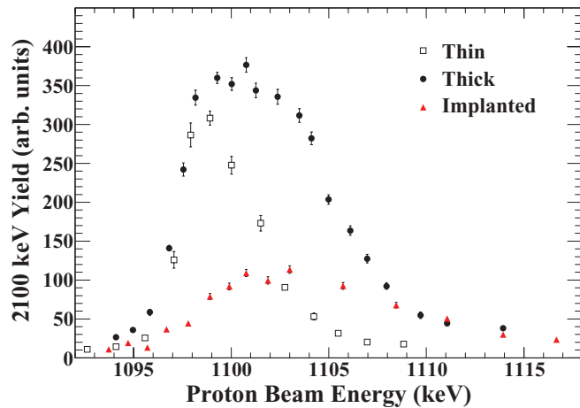
FIG. 2. (Color online) Yield as a function of energy of the 2100 keV \gamma ray from the E_p = 1098 keV ( E_r = 1037 keV) ^{17}\text{O}(p, \gamma)^{18}\text{F} narrow resonance. The three sets of data points correspond to the three different targets used in the experiments.
