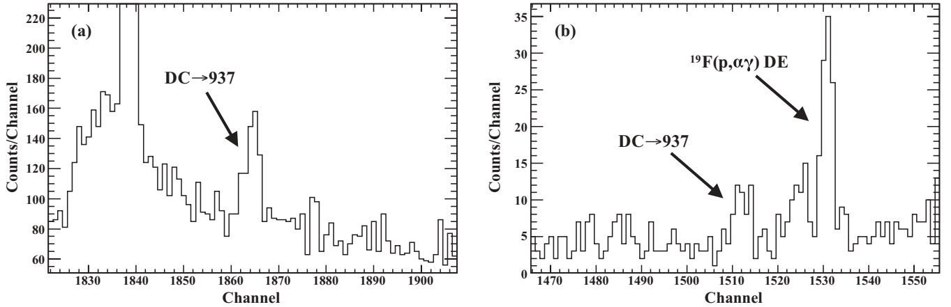
FIG. 4. Spectra of the 45^\circ detector of the angular distribution setup in the energy region of the primary transition to the first excited state in ^{18}\text{F} ( E_x = 937 keV) for proton beam energies of (a) 1625 keV ( E_{\text{c.m.}} = 1535 keV) and (b) 400 keV ( E_{\text{c.m.}} = 378 keV). The low counting statistics of the low-energy spectrum is indicative of the low cross sections, in combination with the detector geometry. The more prominent peaks in both spectra are due to the ^{19}\text{F}(p, \alpha\gamma)^{16}\text{O} reaction, from the fluorine contamination in the tantalum backing.
