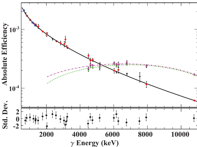
FIG. 5. (Color online) Peak efficiency curves for the 0^\circ detector from the angular distribution experiment. The red circles refer to \gamma -strength measurements of transitions in the ^{27}\text{Al}(p, \gamma)^{28}\text{Si} reaction, the blue squares refer to \gamma -decay measurements with ^{60}\text{Co} and ^{137}\text{Cs} sources, the black triangles relate to \gamma -strength measurements associated with the ^{14}\text{N}(p, \gamma)^{15}\text{O} reaction and the open red circles refer to ^{56}\text{Co} source measurements. The two dashed lines correspond to the single (purple dot-dashed) and double (green dashed) escape peak efficiencies. The bottom graph shows the deviation of the full peak efficiency fit from the data points in units of standard deviation.
