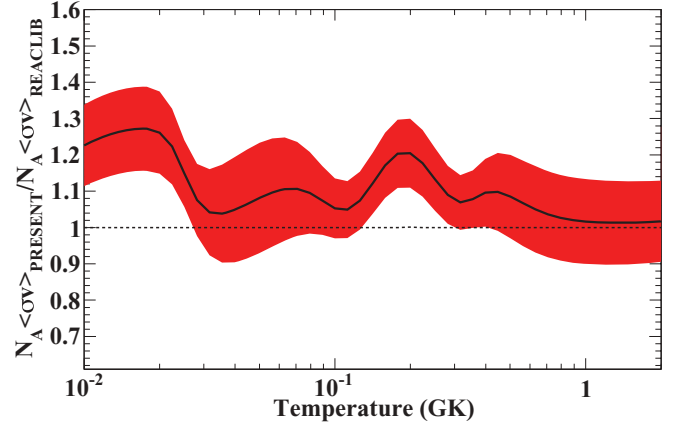
FIG. 12. (Color online) Reaction rate ratio of the present reaction rate to the REACLIB rate as a function of temperature. The uncertainty band includes the estimated uncertainties of the direct capture and resonant components.
