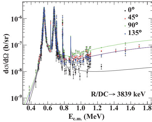
FIG. 8. (Color online) R -matrix fit of the differential cross section of the ^{17}\text{O}(p, \gamma)^{18}\text{F}^*(3839 \text{ keV}) . The different colors and shapes correspond to different angles. The 45^\circ and 135^\circ lines lie on top of each other and cannot be distinguished.
