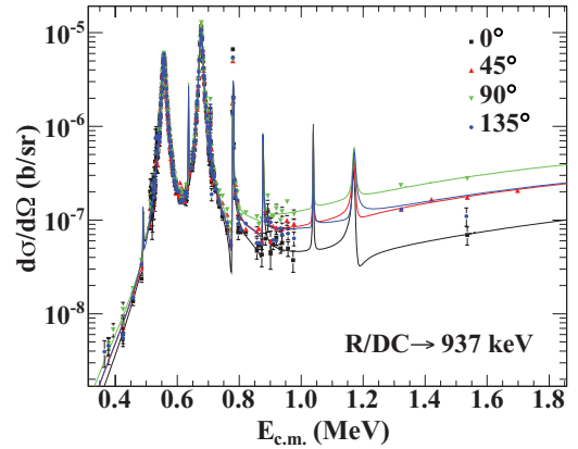
FIG. 7. (Color online) R -matrix fit of the differential cross section of the ^{17}\text{O}(p, \gamma)^{18}\text{F}^*(937 \text{ keV}) . The different colors and shapes correspond to different angles.
