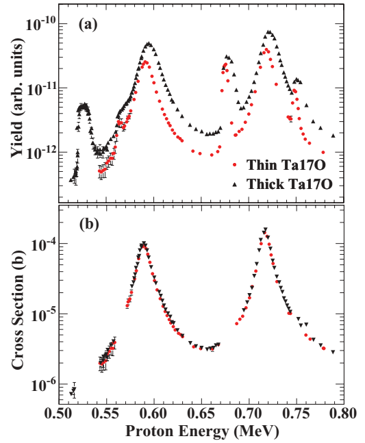
FIG. 6. (Color online) (a) Measured yield of the secondary transition from the first excited state to the ground state of ^{18}\text{F} ( 937 \rightarrow \text{g.s.} ) in the energy region of the two broad resonances. The two data sets correspond to the two anodized targets, \text{Ta}_2\text{O}_5 ‘‘Thin’’ (red circles) and ‘‘Thick’’ (black triangles). (b) Converted yield to cross section with the method described in the text. Narrow resonances were removed in this analysis.
