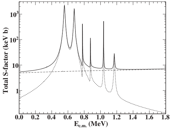
FIG. 9. S factor obtained from the R -matrix fit. The continuous line represents the total S factor from the best R -matrix fit, with background poles included and some ANC values fixed. The dashed-dotted line and the dashed line are the contributions of the direct capture (background poles included) and the high energy resonances, respectively. Some narrow resonances are omitted from this plot.
