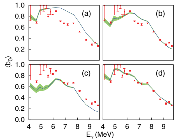
FIG. 3. (Color online) The experimental and calculated \langle b_0 \rangle for four models: (a) the experimental \sigma_{\gamma T} built on excited states (the BH model), (b) the T -dependent width model for the extrapolation of the tail of the GDR for E_x \rightarrow 0 MeV, but using the experimental cross section where it is larger than the extrapolation function, which occurred at about E_\gamma > 5.3 MeV, (c) similar to model (b), but using the GLO model for the GDR, and (d) similar to model (a), but including a resonance built only on excited states between about 5 and 6 MeV, and able to reproduce \langle b_0 \rangle at all energies. The simulation is shown as a solid line and its uncertainty is given by the shaded region.
