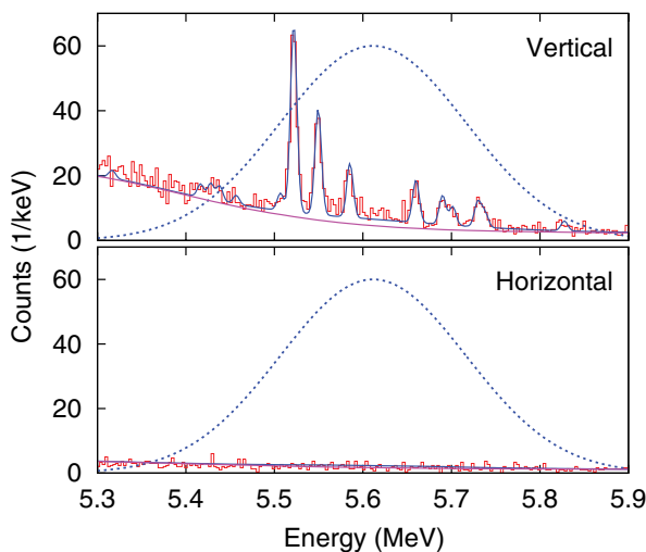
FIG. 1. (Color online) Experimental ^{142}\text{Nd}(\gamma, \gamma') spectra at E_{\text{beam}} = 5.6 MeV. The fit to the peaks and the detector response (primarily the Compton edge) is overlaid. The dashed line is the beam energy profile. The vertical (horizontal) spectrum corresponds to E1 ( M1 ) transitions with a small (4%) overlap of the two angular distributions. Ground-state E1 transitions for several discrete states are seen in the vertical-detector energy spectrum. At this energy, no discrete transitions are seen in the horizontal detectors.
