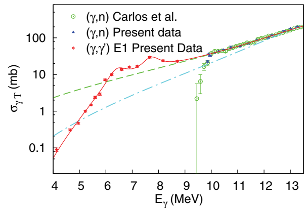
FIG. 2. (Color online) The ^{142}\text{Nd}(\gamma, n) cross section and the E1 photoabsorption cross section \sigma_{\gamma T} . The data from Carlos et al. [28] was scaled by 0.86 [29]. The dashed (dash-dotted) line is a fit to the combined ( \gamma, n ) data using a Lorentzian (temperature-dependent width) function for the GDR [30]. The solid line is a fit to the experimental data.
