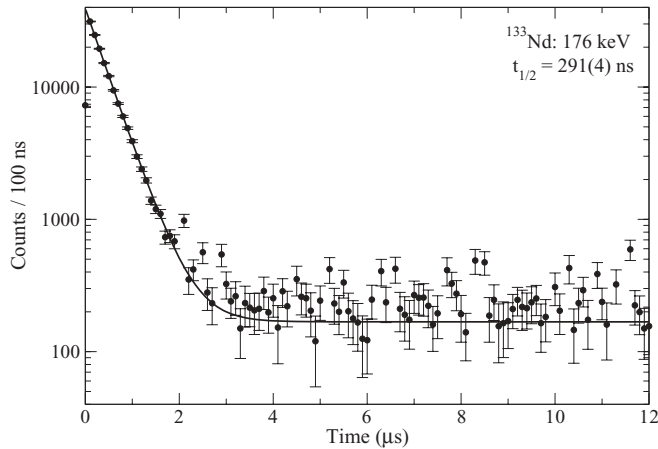
FIG. 2. Recoil- \gamma time distribution for the delayed 176 keV decay in ^{133}\text{Nd} . A least-squares fit yielded a half-life of 291(4) ns.
