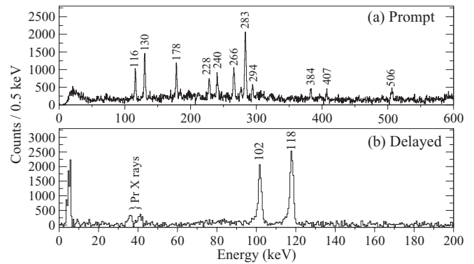
FIG. 4. Spectra produced from a prompt-delayed \gamma - \gamma coincidence matrix for ^{132}\text{Pr} . The matrix had an optimum recoil-delayed \gamma correlation time of 9 \mu\text{s} and was background subtracted. (a) Prompt \gamma rays that correlate with delayed 118 keV decays. (b) Delayed \gamma rays that correlate with prompt 283 keV decays.
