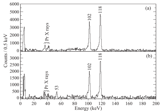
FIG. 5. Planar Ge spectra produced from a prompt-delayed \gamma - \gamma coincidence matrix with a 9 \mu\text{s} recoil-delayed \gamma correlation time (a) gated by the prompt 283, 130, and 266 keV transitions in ^{132}\text{Pr} and (b) gated by the prompt 116, 178, 228, and 277 keV transitions in ^{132}\text{Pr} .
