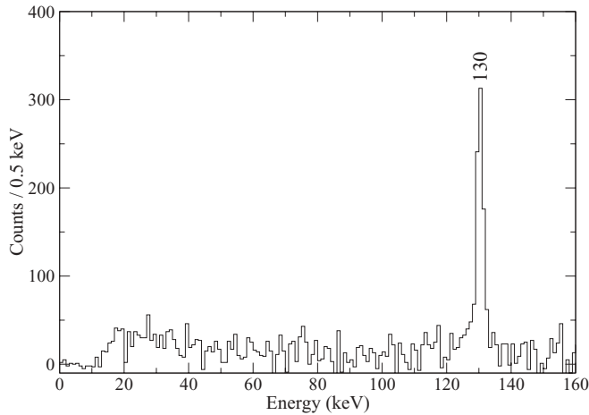
FIG. 8. The low-energy portion of a 283 keV-gated prompt spectrum produced from the 118 keV gated prompt \gamma - \gamma matrix which had a recoil-delayed \gamma time condition of 9 \mu s. The spectrum shows no evidence for correlated decays with energies below the 130 keV transition.
