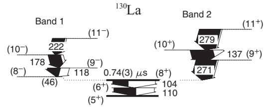
FIG. 12. Partial ^{130}\text{La} decay scheme produced in this work. The newly observed delayed \gamma rays at 104 and 110 keV are tentatively positioned below the proposed (8^+) isomeric state. The weighted mean of the half-lives measured from the 104 and 110 decay time distributions is adopted as the half-life for the (8^+) state. The 46 keV decay was reported in a previous study [12] but not observed in this work.
