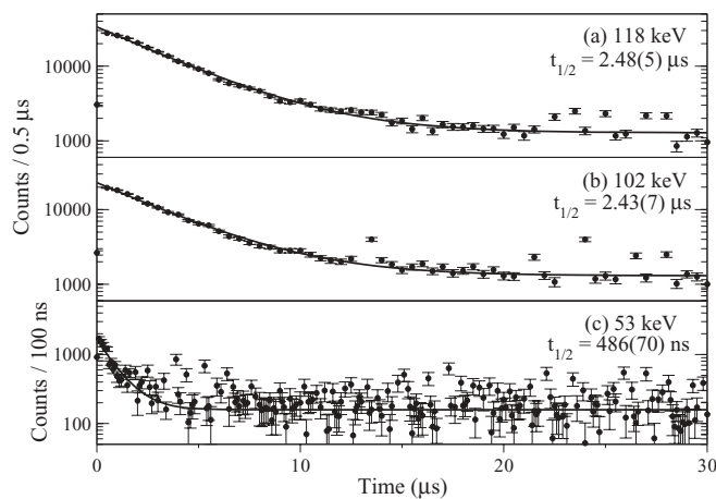
FIG. 3. Recoil- \gamma time distributions for the delayed (a) 118 keV, (b) 102 keV, and (c) 53 keV decays in ^{132}\text{Pr} along with least-squares fit curves.
