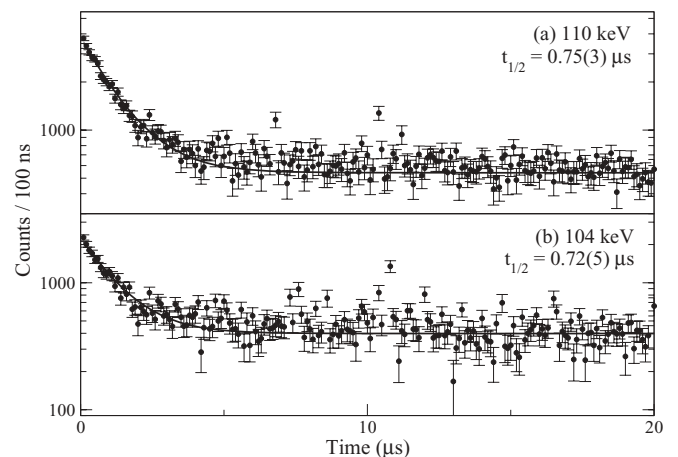
FIG. 9. Recoil- \gamma time distributions for the delayed (a) 110 keV and (b) 104 keV decays in ^{130}\text{La} along with least-squares fit curves.
