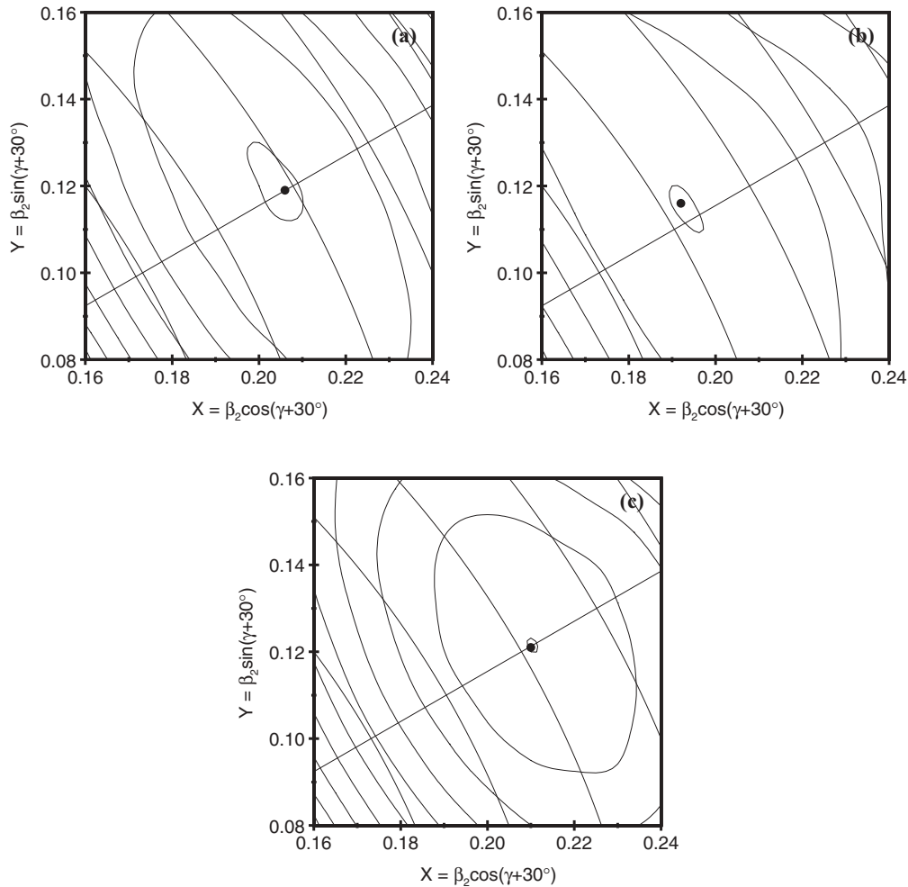
FIG. 13. The results of potential-energy-surface calculations for the proposed (a) \pi 3/2^- [541] \otimes \nu 7/2^+ [404] negative-parity band configuration along with two possible configurations (b) \pi 3/2^- [541] \otimes \nu 7/2^- [523] and (c) \pi 3/2^- [541] \otimes \nu 9/2^- [514] for the positive-parity band in ^{132}\text{Pr} .
