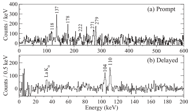
FIG. 10. Spectra produced from a prompt-delayed \gamma - \gamma coincidence matrix for ^{130}\text{La} . The matrix had an optimum recoil-delayed \gamma correlation time of 2.5 \mu\text{s} and was background subtracted. (a) Prompt \gamma rays that correlate with delayed 110 keV decays. (b) Delayed \gamma rays that correlate with prompt 137 keV decays.
