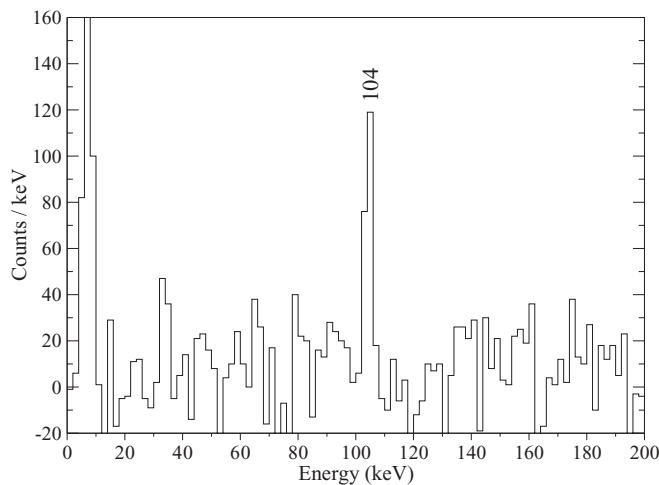
FIG. 11. Background-subtracted planar Ge detector spectrum showing delayed \gamma rays that were in coincidence (within 400 ns) with ^{130}\text{La} 110 keV decays recorded by the focal-plane clover detector. Both planar and clover signals correlated with a recoil implantation within 2.5 \mu\text{s} .
