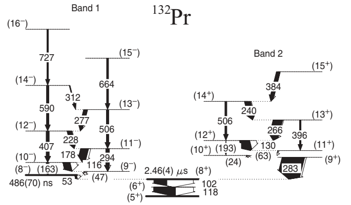
FIG. 7. Partial ^{132}\text{Pr} decay scheme produced in this work. The newly observed delayed \gamma rays at 53, 102, and 118 keV are tentatively positioned below the proposed (8^-) and (8^+) isomeric states. The weighted mean of the half-lives measured from the 102 and 118 decay time distributions is adopted as the half-life for the (8^+) state. Bracketed decays were reported in a previous study [14] but not observed in this work.
