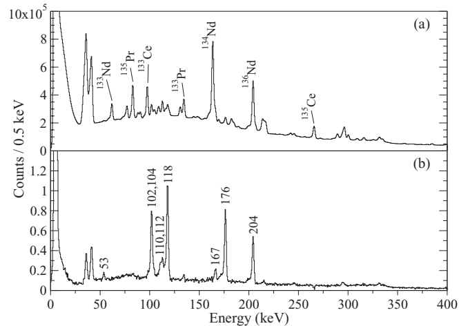
FIG. 1. Planar Ge detector spectra showing recoil-correlated delayed \gamma rays. (a) \gamma rays recorded within 40 \mu\text{s} of a recoil implantation. The majority of the transitions result from states populated by \beta decay, the most intense of which are labeled with the parent nucleus. (b) \gamma rays recorded within 11 \mu\text{s} of a recoil implantation. A random-correlation background spectrum of \gamma rays, recorded up to 11 \mu\text{s} prior to the recoil signal, was subtracted.
