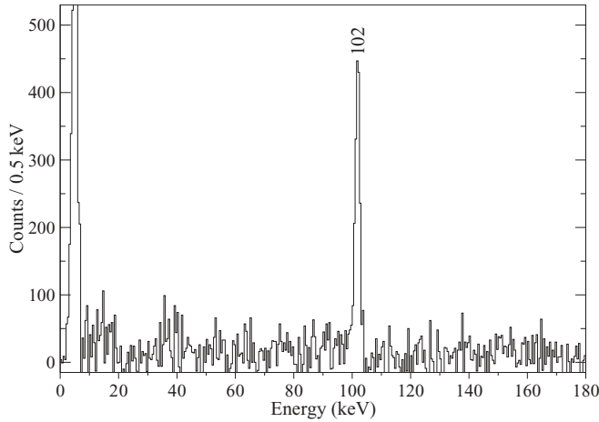
FIG. 6. Background-subtracted planar Ge detector spectrum showing delayed \gamma rays that were in coincidence (within 400 ns) with ^{132}\text{Pr} 118 keV decays recorded by the focal-plane clover detector. Both planar and clover signals correlated with a recoil implantation within 9 \mu\text{s} .
