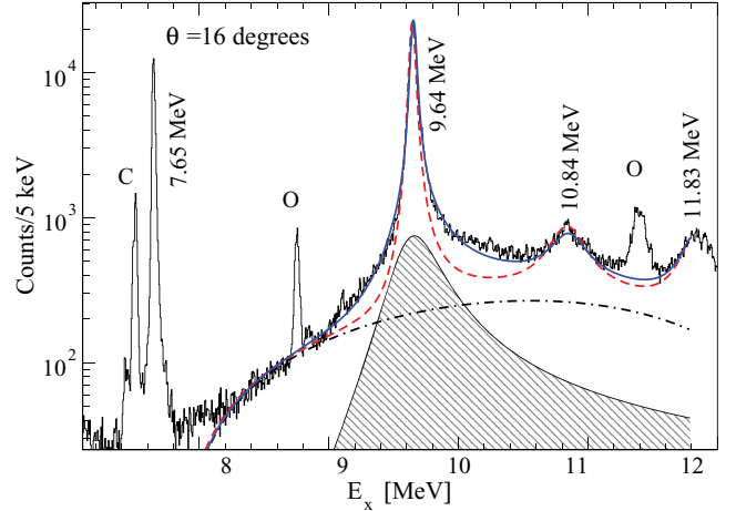
FIG. 3. (Color online) ^{12}\text{C} excitation energy spectrum from a measurement of proton inelastic scattering for a 66 MeV proton beam and a scattering angle of \theta_{\text{lab}} = 16^\circ . Contaminants from ^{13}\text{C} and ^{16}\text{O} target contaminants are labeled C and O, respectively. Two fits are shown. The red dashed line corresponds to all known ^{12}\text{C} states. The solid blue curve includes an additional 2^+ contribution from an R -matrix calculation. The hatched region shows the asymmetric shape of the 2^+ state predicted by the R -matrix calculation [Eq. (1)], see text for details. The black dot-dashed line is the scaled broad 0^+ background used in the fit which includes the proposed 2^+ contribution.
