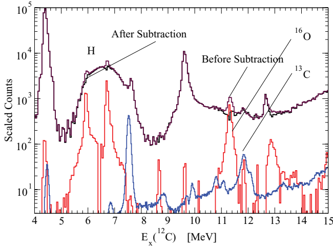
FIG. 2. (Color online) Analysis of background contributions to the ^{12}\text{C} excitation energy spectrum populated in \alpha -inelastic scattering at \theta_{\text{lab}} = 3.7^\circ . The maroon histogram (labeled “Before Subtraction”) is the data before background subtraction. The hydrogen contaminant is labeled H. The red histogram (labeled “ ^{16}\text{O} ”) shows the ^{16}\text{O} contaminant spectrum, which when subtracted gives the black histogram (labeled “After Subtraction”). The blue histogram (labeled “ ^{13}\text{C} ”) shows a measurement of ^{13}\text{C}(\alpha, \alpha') measured at \theta_{\text{lab}} = 3.7^\circ [19]. The broad feature in the ^{12}\text{C} excitation energy spectrum between 9 and 10 MeV cannot be interpreted in terms of target contaminants.
