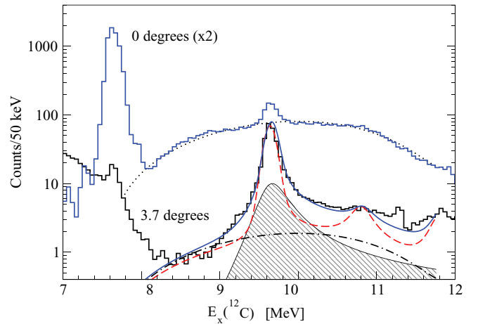
FIG. 1. (Color online) {}^{12}\text{C} excitation energy spectra (with the {}^{16}\text{O} background subtracted) from \alpha -particle inelastic scattering at 386 MeV at \theta_{\text{lab}} = 0 and 3.7^\circ . The black-dotted curve characterizes the shape of the 10.3 MeV 0^+ state (and any other broad components). The data at \theta_{\text{lab}} = 3.7^\circ have been fitted with two curves. The red dashed line corresponds to all known {}^{12}\text{C} states. The solid blue curve includes an additional 2^+ contribution from an R -matrix calculation. The hatched region shows the asymmetric shape of the 2^+ state predicted by the R -matrix calculation [Eq. (1)], see text for details. Note there is a contaminant from the hydrogen in the target between 5 and 8 MeV (labeled H in Fig. 2.) The black dot-dashed line is the scaled broad 0^+ background used in the fit which includes the proposed 2^+ contribution.
