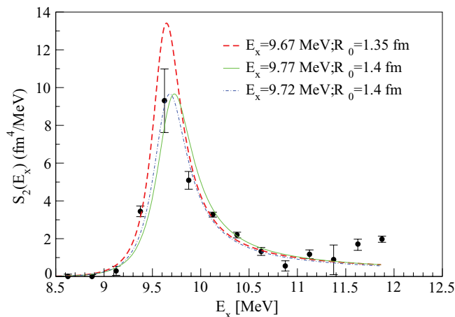
FIG. 4. (Color online) The spin-2 strength function [S_2(E_x)] extracted from the multipole decomposition analysis [17] (data points) compared with the R -matrix line shapes [Eq. (1)] associated with different channel radii and excitation energies.
