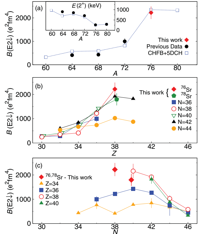
FIG. 3. (Color online) (a) Experimental values of B(E2 \downarrow) and E(2^+) (inset) for the N = Z nuclei are compared to predictions from the CHFB + 5DCH calculations [16]. The B(E2 \downarrow) values in the vicinity of ^{76}\text{Sr} are also plotted in the (b) isotonic and (c) isotopic chains. Data are taken from Refs. [3,5–7,28,29].
