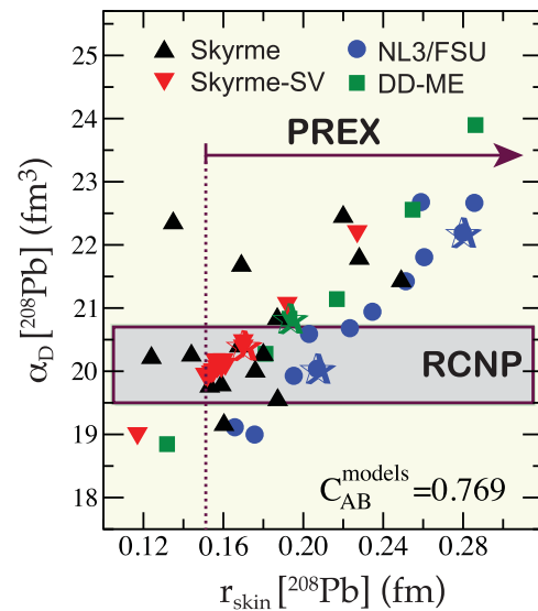
FIG. 1. (Color online) Predictions from 48 nuclear EDFs discussed in the text for the electric dipole polarizability and neutron-skin thickness of ^{208}\text{Pb} . Constrains on the neutron-skin thickness from PREX [3] and on the dipole polarizability from RCNP [27] have been incorporated into the plot.
