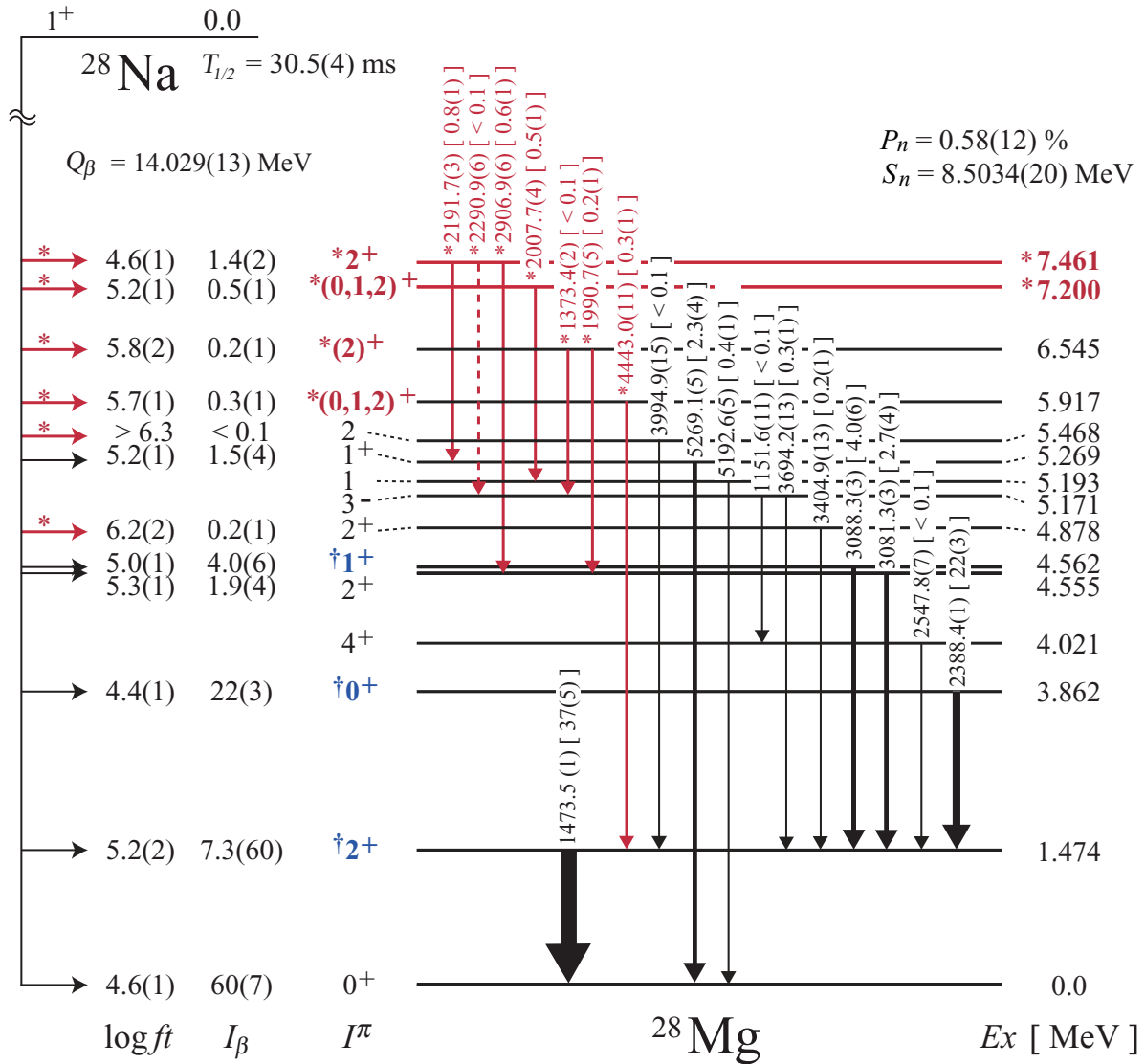
FIG. 6. (Color online) Revised decay scheme of ^{28}\text{Na} . The level energies are re-evaluated. Newly found transitions and energy levels as well as newly assigned spins and parities are labeled by asterisks. The spins and parities labeled by daggers denote that these assignments are reconfirmed in the present work. Reported values of T_{1/2} [33], Q_\beta [34], P_n [33], and S_n [34] are also shown.
