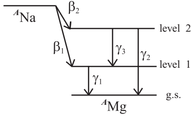
FIG. 3. Schematic decay scheme of a neutron-rich ^4\text{Na} isotope.
