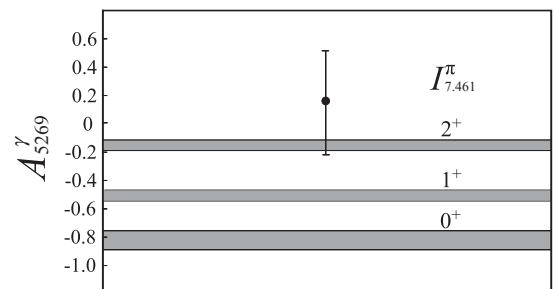
FIG. 9. Asymmetry parameter A_{5269}^{\gamma} of \beta decay in coincidence with the 5269-keV \gamma ray. The experimental result is shown by the closed circle and the shaded area corresponds to the expected A_{5269}^{\gamma} values for the assumed spin-parity of the 7.461-MeV level.
