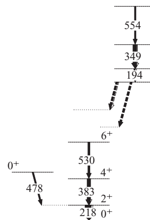
FIG. 9. Partial energy level scheme for ^{194}\text{Os} (from [44]) showing decay \gamma rays observed in the present work following the \beta^- decay of ^{194}\text{Re} .
