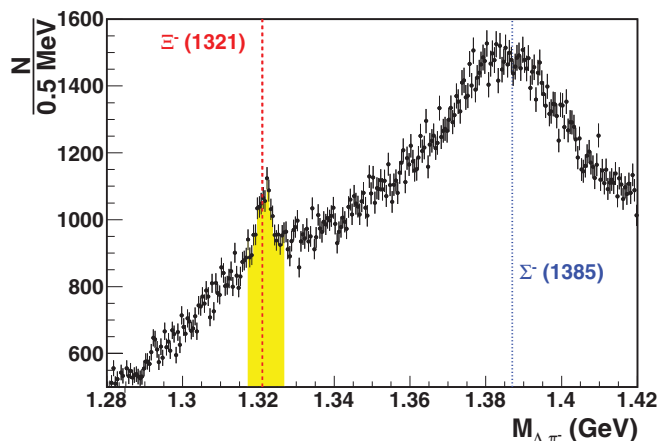
FIG. 4. (Color online) Invariant mass of the \Lambda\pi^- pairs. The red dashed and blue dotted lines mark the positions of the nominal mass for \Xi^-(1321) and \Sigma^-(1385) , respectively [4]. The shaded area shows the mass range used in this analysis.
