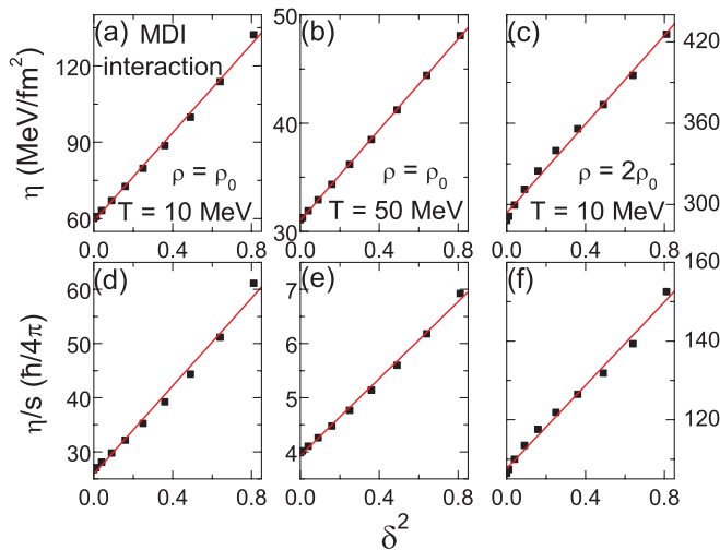
FIG. 6. (Color online) Shear viscosity \eta and specific viscosity \eta/s as functions of isospin asymmetry \delta^2 for different densities and temperatures. The solid lines are from the linear fit.
