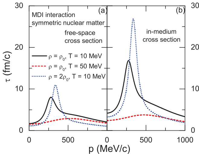
FIG. 4. (Color online) Momentum dependence of the total relaxation time at different densities and temperatures in symmetric nuclear matter from free-space cross sections (a) and in-medium cross sections (b).
