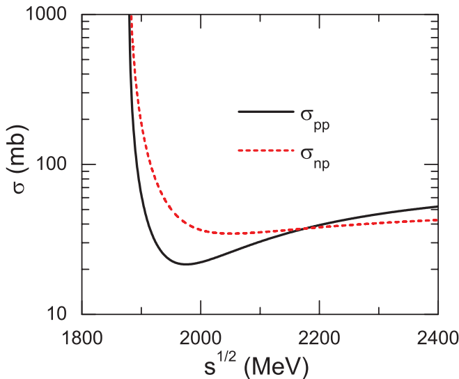
FIG. 2. (Color online) pp and np cross sections in free space as functions of the center-of-mass energy of the two colliding nucleons from the parametrized form [Eqs. (21) and (22)].
