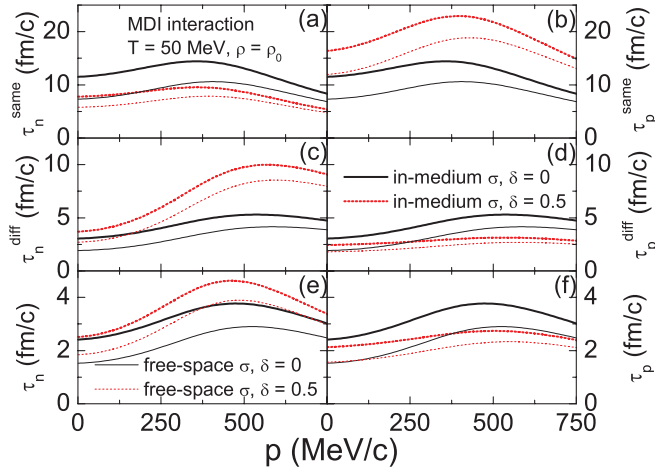
FIG. 3. (Color online) Momentum dependence of the total relaxation time and the relaxation time for the nucleon to collide with other ones of same or different isospin in symmetric ( \delta = 0 ) and neutron-rich ( \delta = 0.5 ) nuclear matter.
