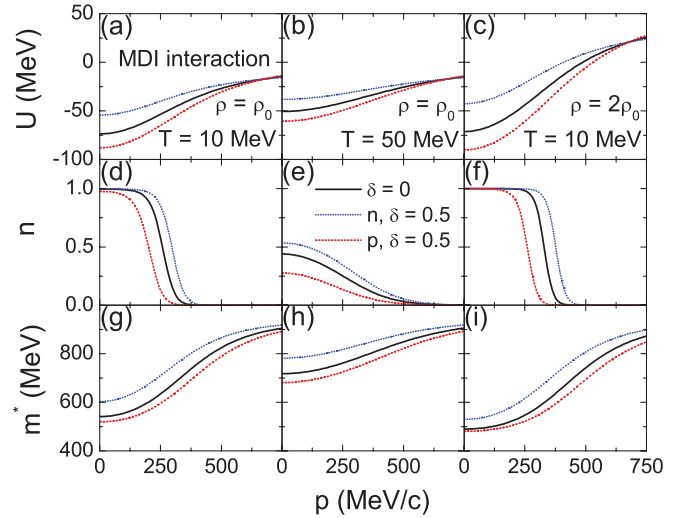
FIG. 1. (Color online) Momentum dependence of the single-particle potential, the occupation probability, and the effective mass at \rho = \rho_0 and T = 10 MeV [(a), (d), (g)], \rho = \rho_0 and T = 50 MeV [(b), (e), (h)], and \rho = 2\rho_0 and T = 10 MeV [(c), (f), (i)] from the MDI interaction. Results from symmetric ( \delta = 0 ) nuclear matter and neutron-rich ( \delta = 0.5 ) nuclear matter are compared.
