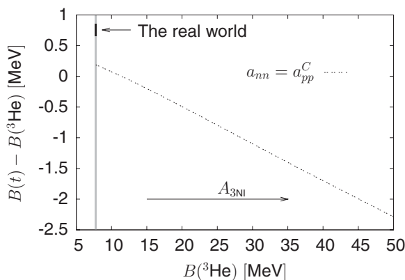
FIG. 5. Difference between binding energies for the mirror nuclei t and ^3\text{He} as a function of the ^3\text{He} binding energy at a_{nn} = a_{pp}^C .
