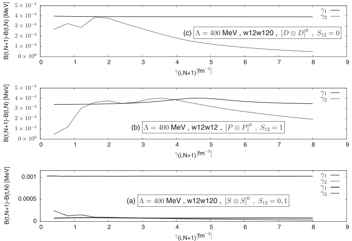
FIG. 6. Difference in B(t) due to the addition of basis vectors to a reference set w12w12(0). This change is shown in the lowest panel (a) as a function of either of the two width parameters \gamma_{1,2} for a d - n ( d - n ) grouping in two S waves. (b) The change for the nucleons in relative P waves. (c) The change for the nucleons in relative D waves.
