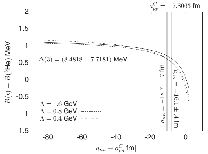
FIG. 2. Correlation between the trinucleon-binding-energy difference B(t) - B(^3\text{He}) and the nn and pp scattering lengths at LO in EFT( \pi ). Correlation lines correspond to regulator values of 400 MeV, 800 MeV, and 1.6 GeV with B(d) as input. For \Lambda = 700 MeV, the correlations overlap with the displayed lines and are not shown.
