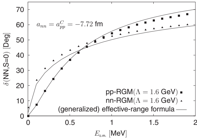
FIG. 4. Comparison between the analytic (generalized) effective range formula ([59]) and the cutoff ( \Lambda = 1.6 GeV) RGM predictions with EFT( \not\hbar ) for the ( pp ) nn ^1S_0 scattering phase shift with a_{nn} = a_{pp}^C .
