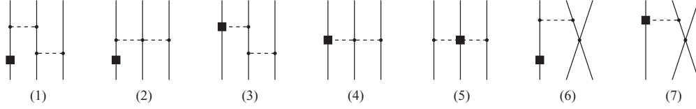
FIG. 3. Tree diagrams contributing to the two-pion-exchange and one-pion-exchange-contact topology of the 3NF at N^3\text{LO} . The solid boxes denote insertions of either subsubleading d_i vertices from the effective pion-nucleon Lagrangian or the leading 1/m corrections. For notation see Fig. 1.
