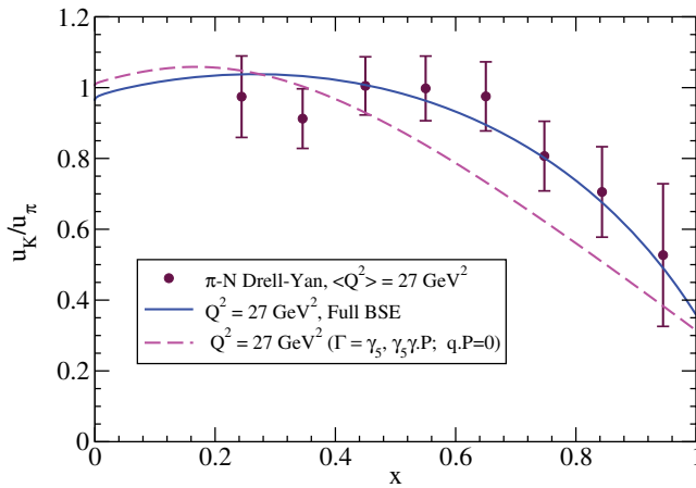
FIG. 4. (Color online) DSE prediction for the ratio of u -quark distributions in the kaon and pion [5,31]. The full Bethe-Salpeter amplitude produces the solid curve; the reduced BS amplitude produces the dashed curve. The reduced amplitude retains only the invariants and amplitudes involving pseudoscalar and axial vector Dirac matrices, and ignores dependence on the variable q \cdot P . These are part of the reductions that occur in a pointlike treatment of the pseudoscalar mesons. The experimental data are from [1,4].
