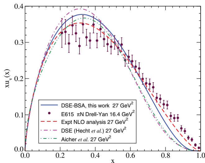
FIG. 2. (Color online) Pion valence quark distribution function evolved to (5.2 \text{ GeV})^2 . Solid curve: full DSE calculation [31]; dot-dashed curve: semi-phenomenological DSE-based calculation in Ref. [18]; filled circles: experimental data from Ref. [3], at scale (4.05 \text{ GeV})^2 ; dashed curve: NLO reanalysis of the experimental data [32]; and dot-dot-dashed curve: NLO reanalysis of experimental data with inclusion of soft-gluon resummation [33].
