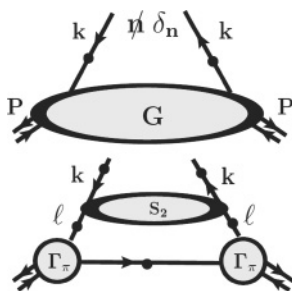
FIG. 1. Diagrammatic representation of parton distributions. Top panel: the exact parton distribution corresponding to Eq. (2). Bottom panel: Rainbow-ladder truncation of the amplitude G . S_2 is the q\bar{q} propagator.
