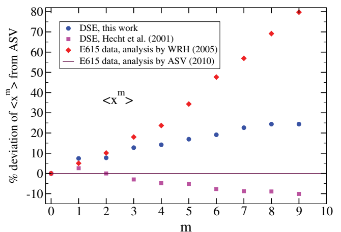
FIG. 3. (Color online) Moments of the pion's valence u(x) at scale (5.2 \text{ GeV})^2 , shown as a percent deviation from the recent (ASV) reanalysis [33] (NLO, with soft gluon resummation) of the 1989 E615 \pi N Drell-Yan data [3]. Filled circles: present full DSE calculation [31]; filled squares: semi-phenomenological DSE-based calculation [18]; and filled diamonds: reanalysis (NLO, without soft gluon resummation) of the same Drell-Yan data [32].
