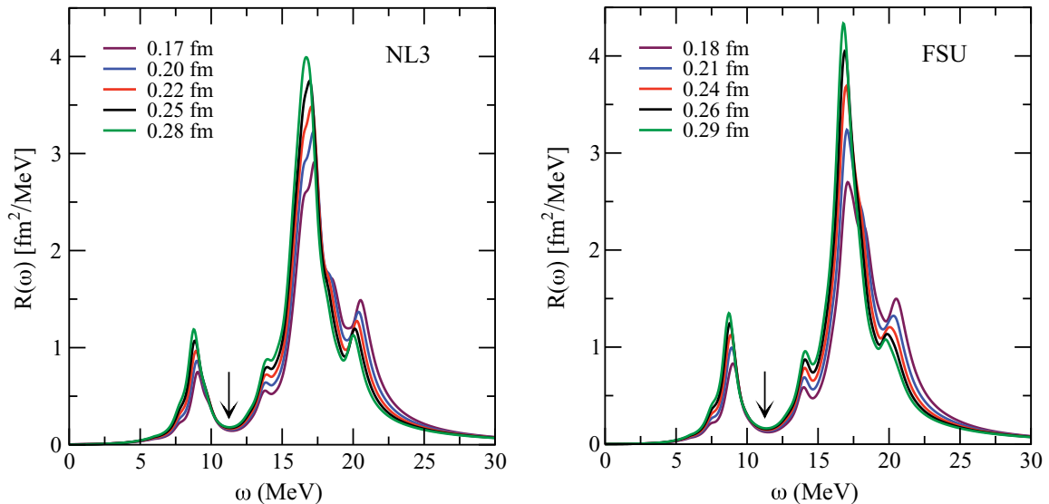
FIG. 4. (Color online) Distribution of dipole strength in ^{68}\text{Ni} computed in an MF + RPA approach using the NL3 (left panel) and FSU (right panel) families of effective interactions.
