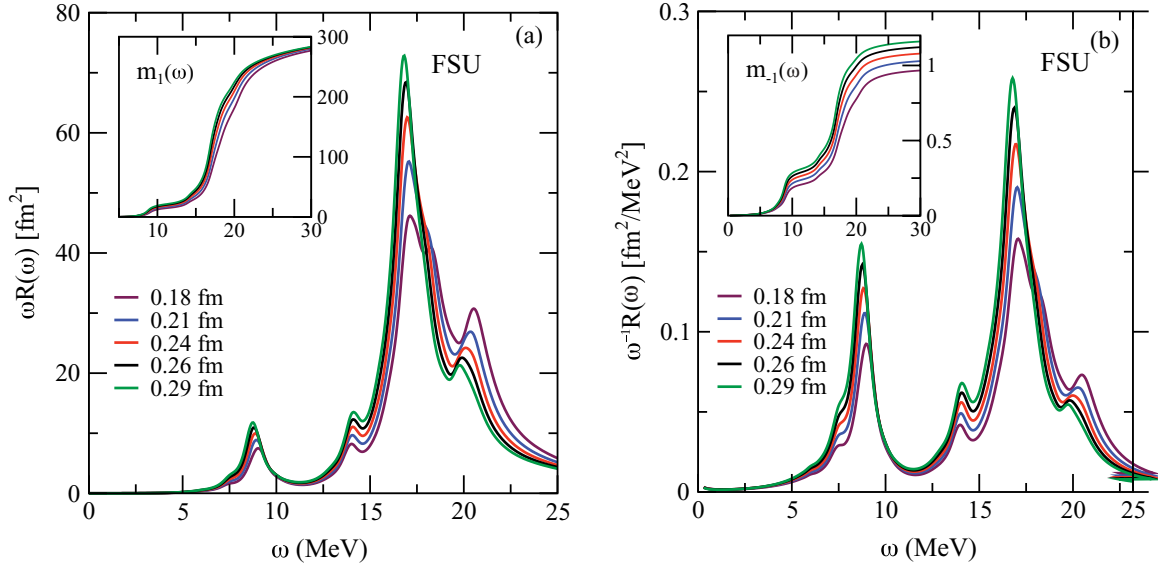
FIG. 5. (Color online) The energy-weighted dipole response (a) and the inverse energy-weighted dipole response (b) in ^{68}\text{Ni} computed with the FSU family of effective interactions. The insets display the cumulative sums, as defined in Eqs. (14) and (15).
