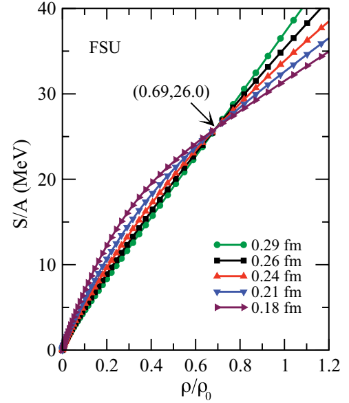
FIG. 2. (Color online) Symmetry energy per nucleon as a function of density (in units of the saturation density). The various effective interactions are labeled according to their predictions for the neutron-skin thickness of ^{208}\text{Pb} .
