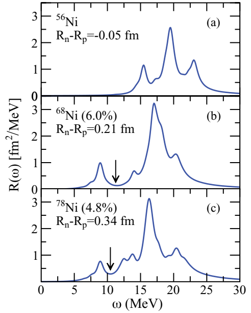
FIG. 1. (Color online) Distribution of isovector dipole strength for the three closed-(sub)shell nickel isotopes ^{56}\text{Ni} , ^{68}\text{Ni} , and ^{78}\text{Ni} . Mean-field-plus-RPA predictions are shown, using the FSUGold parameter set [53].
