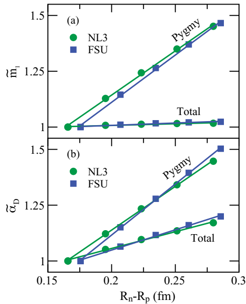
FIG. 6. (Color online) Fractional changes in the energy-weighted sum (a) and dipole polarizability (b) for ^{68}\text{Ni} as a function of the neutron-skin thickness of ^{208}\text{Pb} .
