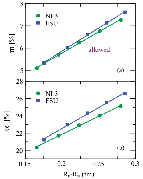
FIG. 7. (Color online) Percentages of the energy-weighted sum (a) and the dipole polarizability (b) exhausted by the pygmy dipole resonance in ^{68}\text{Ni} as a function of the neutron-skin thickness of ^{208}\text{Pb} .
