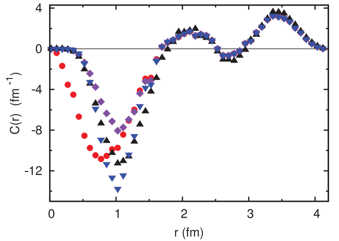
FIG. 4. (Color online) The radial functions C(r) from Eq. (8) that represent the contribution of internucleon distance r to the 0\nu\beta\beta matrix element. Each curve corresponds to one of the distributions P_F(r) of Fig. 3. (The P_{GT} are just proportional to the P_F for the simple spin-zero pairs in our wave function.) The symbols indicate the same approximations as in Fig. 3.
