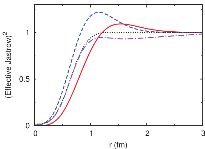
FIG. 1. (Color online) Squares of Jastrow functions F_{ab} from calculations following Ref. [13] (dotted black line, spin-singlet only), from Miller and Spencer [3] (solid red line), and from a fit to the results of a microscopic Brueckner-based calculation [9] (dashed blue line). The purple dot-dashed line comes from three-body and higher corrections to the dotted line.
