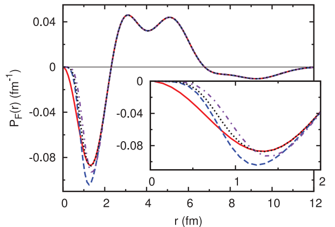
FIG. 2. (Color online) The charge-changing two-body density P_F(r) for the shell-model calculation of ^{82}\text{Se} in Refs. [15] and [16]. The solid red line is the result without short-range correlations, the dashed blue line is that from the Brueckner-based calculation of Ref. [8], the dotted black line applies the Jastrow function from the approach in Ref. [13] in the two-body cluster approximation, and the dot-dashed purple line applies the Miller-Spencer Jastrow function. The inset magnifies the left-hand part of the figure.
