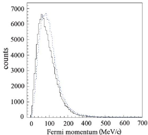
FIG. 7. (Color online) Fermi momentum (dashed line) of the neutron after the cuts (data) and Fermi momentum (solid line) generated using the Paris potential.
