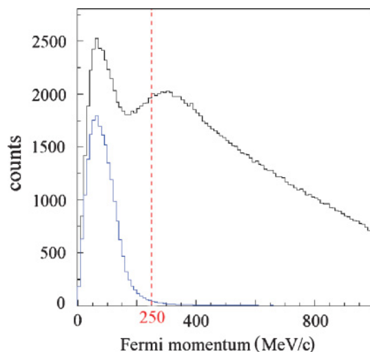
FIG. 6. (Color online) Fermi momentum of the neutron calculated before (upper curve) and after (lower curve) the cuts.
