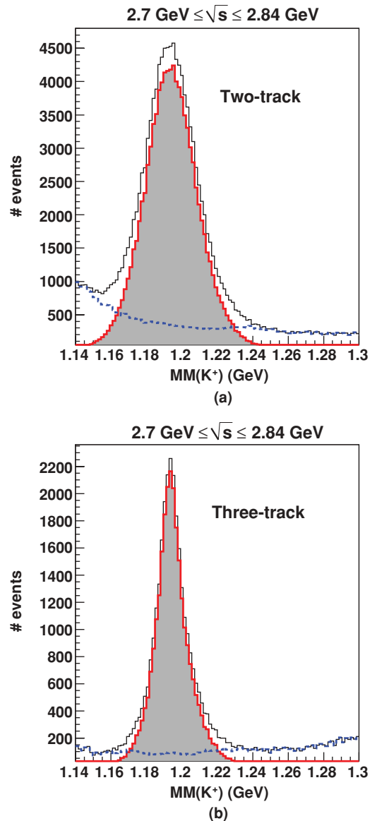
FIG. 5. (Color online) Signal-background separation in the high \sqrt{s} regions integrated over all angles for (a) two-track and (b) three-track topologies. The red (shaded) histograms are the data weighted by Q , representing the signal, while the blue (dotted) histograms are the data weighted by (1 - Q) , representing the background. Note that the three-track data set has a smaller background from the K^+\Lambda “tail” because of the additional cut described in subsection IV B.
