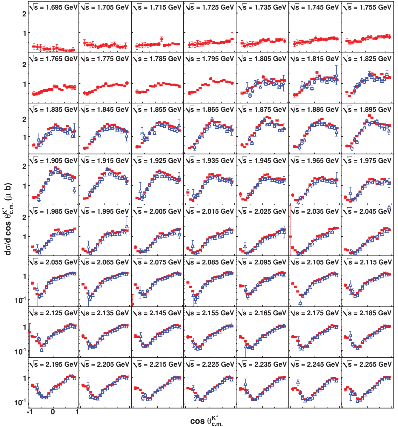
FIG. 8. (Color online) \frac{d\sigma}{d \cos \theta_{c.m.}^{K^+}} ( \mu\text{b} ) vs. \cos \theta_{c.m.}^{K^+} : Differential-cross-section results for the two topologies in the energy range 1.69 \text{ GeV} \leq \sqrt{s} < 2.26 \text{ GeV} . The centroid of each 10-MeV-wide bin is printed on the plots. Results from the two-track analysis are represented by red squares, and those from the three-track analysis by blue triangles. Note that we do not present results in the \sqrt{s} = 1.955 \text{ GeV} bin (see Sec. VII) and that the y axes are set to logarithmic scales from \sqrt{s} = 2.055 \text{ GeV} onward. All error bars represent statistical uncertainties only.
