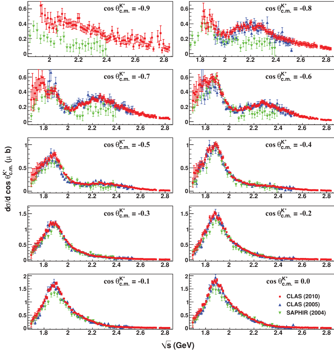
FIG. 10. (Color online) \frac{d\sigma}{d \cos \theta_{c.m.}^{K^*}} (\mu\text{b}) vs. \sqrt{s} in the backward angles: final CLAS (present analysis) differential-cross-section results as the weighted average of the two topologies are in red squares. Previous CLAS results [14] are in blue up-triangles while green down-triangles are results from SAPHIR [16]. All error bars represent statistical uncertainties only.
