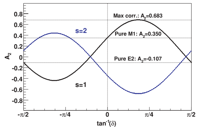
FIG. 13. (Color online) Neutron- \gamma correlation as a function of the M1/E2 admixture ( \delta ) for channel spins s = 1 (black solid line) and s = 2 (blue dotted line). The x axis is expressed as \tan^{-1}(\delta) to show the pure E2 case ( |\delta| \rightarrow \infty ). The significant A_2 values for channel spin s = 1 are highlighted (see text).
