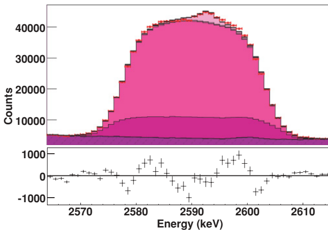
FIG. 11. (Color online) Line-shape analysis of the (1^-, 2_2^+) \rightarrow 2_1^+ doublet transition without n - \gamma correlations. The best fit is obtained using the parameters given in Tables VIII and VII. The relative contribution of each contributing branch is shown by using different shades of purple. The difference between the experimental data and the simulation is shown below the figure.
