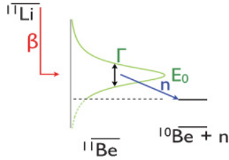
FIG. 3. (Color online) Schematic of neutron emission from an excited state in ^{11}\text{Be} . The state is modeled as a Breit-Wigner distribution (green solid line), with centroid E_0 and width \Gamma . The low-energy tail in the dotted line shows the part of the distribution truncated to forbid negative neutron energies.
