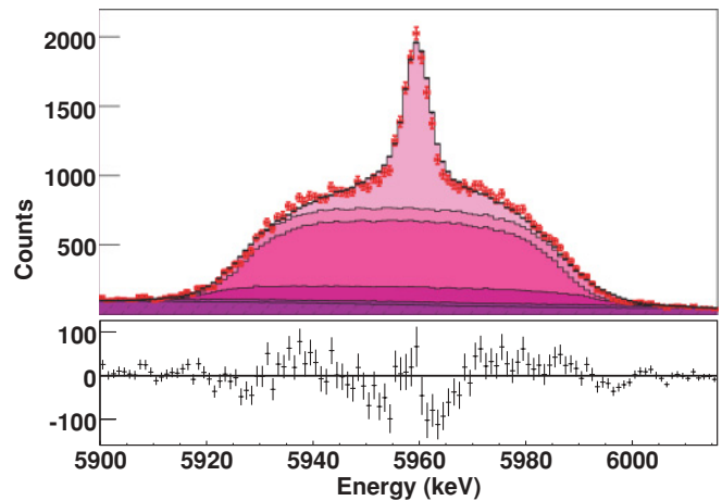
FIG. 12. (Color online) Same as Fig. 11, but for the (1^-, 2_2^+) \rightarrow 0_1^+ doublet transition without n - \gamma correlations.
