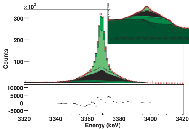
FIG. 14. (Color online) Line-shape analysis of the 2_1^+ \rightarrow 0_1^+ 3367-keV transition. The best fit is obtained using the parameters given in Table IX. The inset shows the same line shape shown on a log scale to reveal the higher lying neutron contributing branches. In both pictures, the relative contribution of each direct neutron branch is shown using different shades of green, except for the sum of all the indirect contributions shown in black. The difference between the experimental data and the simulation is shown below the figure.
