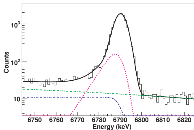
FIG. 4. (Color online) Fit of the 6790-keV transition in ^{11}\text{B} using Eq. (1) plus an additional linear background. The components of the fit are shown in dashed lines of different colors.
