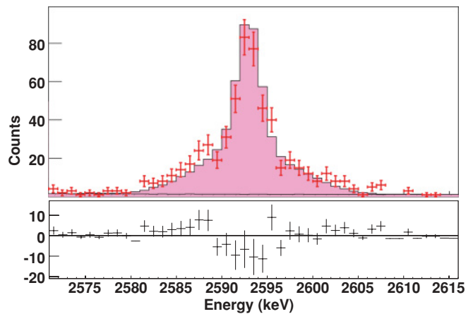
FIG. 9. (Color online) Line-shape analysis of the 1^- \rightarrow 2_1^+ transition isolated by gating on the 0_2^+ \rightarrow 1^- transition. The difference between the experimental data and the simulation is shown below the figure.
