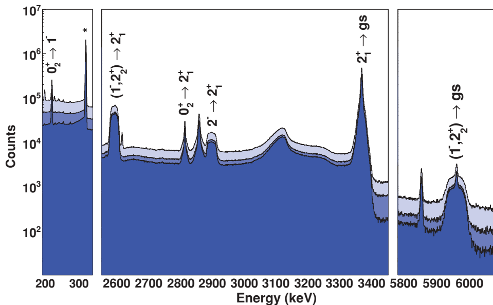
FIG. 1. (Color online) \gamma spectrum recorded following the \beta decay of ^{11}\text{Li} . Shown only are energy sections where ^{10,11}\text{Be} \gamma transitions are present. \gamma singles, \beta - \gamma , and bremsstrahlung-vetoed \beta - \gamma coincidences are displayed in increasingly darker shades of blue. The transition marked with a star (*) is the 320-keV 1/2^- \rightarrow 1/2^+ transition in ^{11}\text{Be} . The other transitions belong to the decay of ^{10}\text{Be} excited states.
