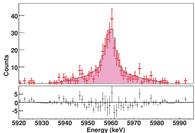
FIG. 10. (Color online) Same as Fig. 9, but for the 1^- \rightarrow 0_1^+ transition isolated by gating on the 0_2^+ \rightarrow 1^- transition.
