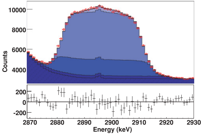
FIG. 6. (Color online) Line-shape analysis of the 2897-keV 2^- \rightarrow 2_1^+ transition. The best fit is obtained using the parameters given in Table V. The relative contribution of each neutron branch is shown by using different shades of blue. The difference between the experimental data and the simulation is shown below the figure.
