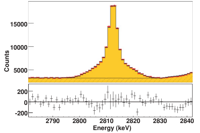
FIG. 7. (Color online) Line-shape analysis of the 2812-keV 0_2^+ \rightarrow 2_1^+ transition. The best fit is obtained using the parameters given in Table VI. The difference between the experimental data and the simulation is shown below the figure.
