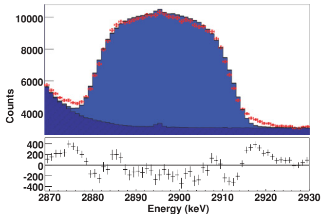
FIG. 5. (Color online) Line-shape analysis of the 2897-keV 2^- \rightarrow 2_1^+ transition using only the 8.82-MeV neutron-emitting state in ^{11}\text{Be} . The difference between the experimental data and the simulation is shown below the figure.
