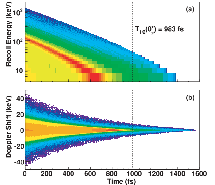
FIG. 8. (Color online) (a) Evolution of the ^{10}\text{Be} recoil energy as a function of time after the neutron emission ( t = 0 ). (b) Evolution of the Doppler broadening as a function of the same time.
