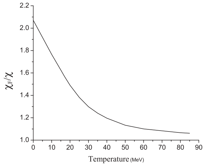
FIG. 4. The magnetic susceptibility of the hot nuclear matter versus the temperature at \rho = 0.16 \text{ fm}^{-3} .
