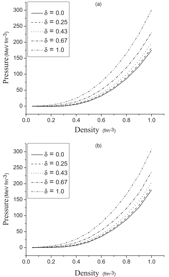
FIG. 8. The equation of state of the polarized hot nuclear matter for different values of the spin polarization ( \delta ) at T = 10 (a) and T = 20 \text{ MeV} (b).
