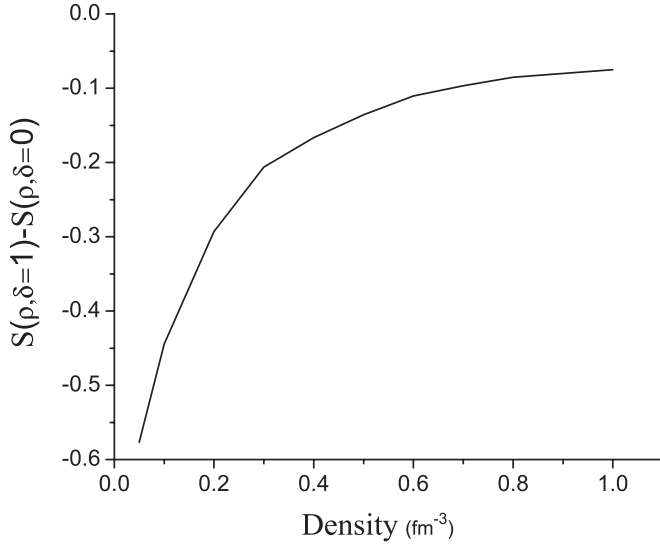
FIG. 6. As in Fig. 4 but for the entropy difference of the fully polarized and the unpolarized cases.
