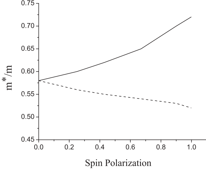
FIG. 1. The effective mass of spin-up (full curve) and spin-down (dashed curve) nucleons versus the spin polarization ( \delta ) for density \rho = 0.5 \text{ fm}^{-3} at T = 20 \text{ MeV} .
