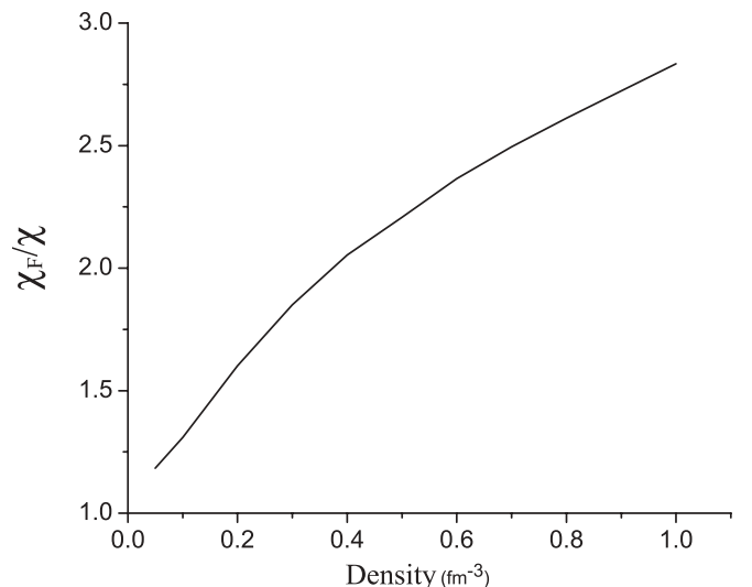
FIG. 5. The magnetic susceptibility of the hot nuclear matter versus the total number density ( \rho ) at T = 20 \text{ MeV} .
