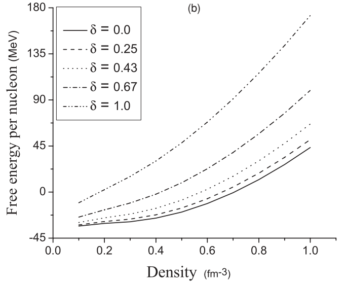
FIG. 2. The free energy per nucleon of the polarized hot nuclear matter as a function of the total number density ( \rho ) for different values of the spin polarization ( \delta ) at T = 10 (a) and T = 20 \text{ MeV} (b).
