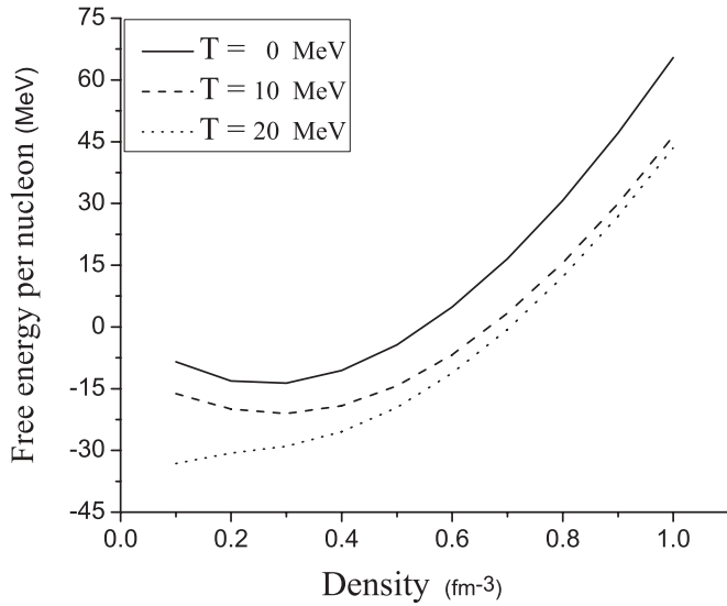
FIG. 3. The free energy per nucleon of the nuclear matter versus the total number density ( \rho ) for unpolarized case at T = 0, 10, and 20 MeV.
