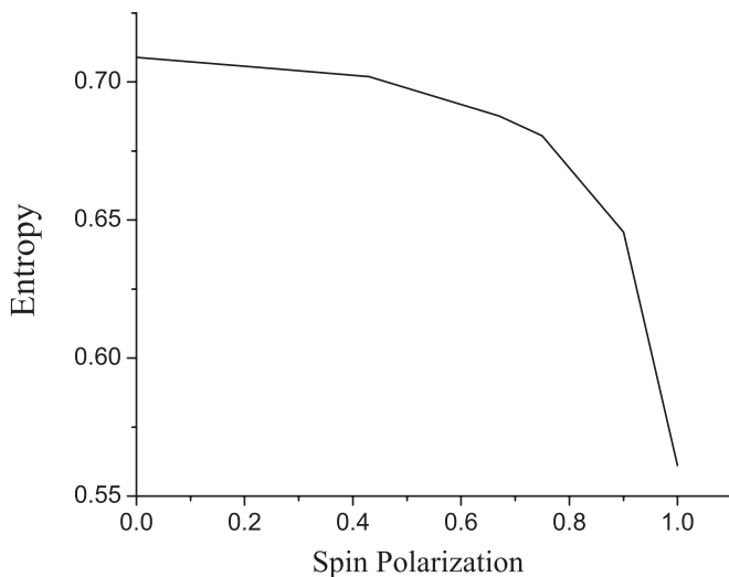
FIG. 7. The entropy per nucleon as a function of the spin polarization ( \delta ) for density \rho = 0.5 \text{ fm}^{-3} at T = 20 \text{ MeV} .
