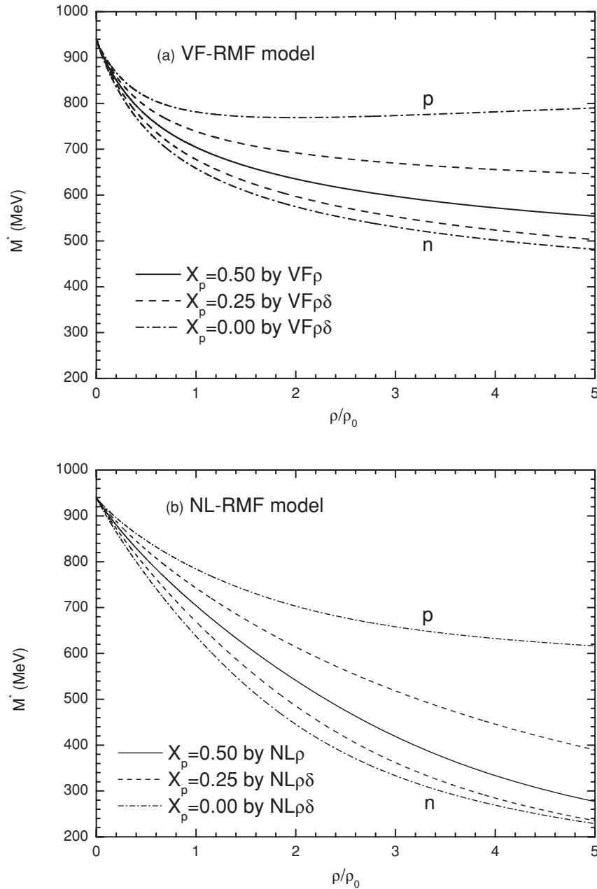
FIG. 3. Nucleon effective masses as a function of the baryon density in different models. The upper (lower) dashed and dash-dotted lines correspond to the masses of the proton (neutron). (a) VF-RMF model. (b) NL-RMF model.
