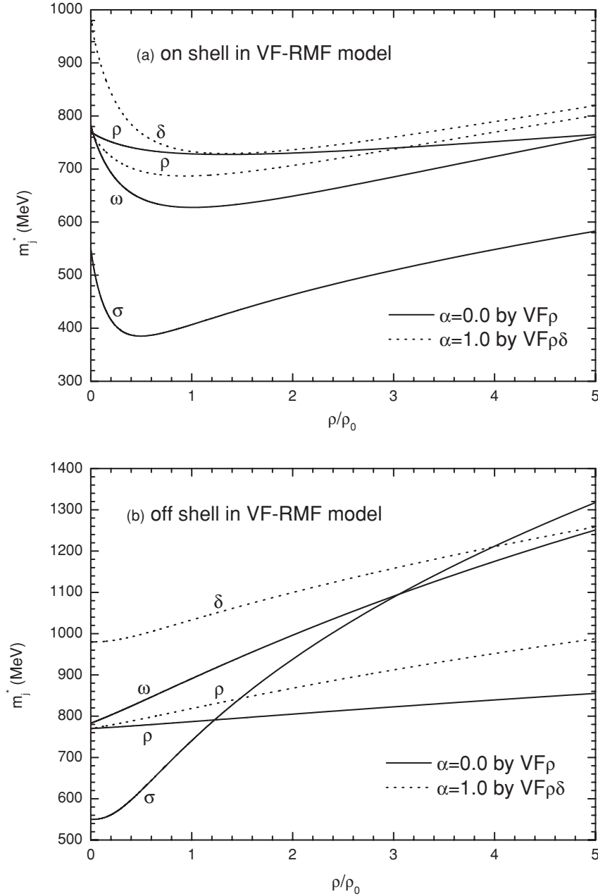
FIG. 2. Meson effective masses as a function of the baryon density in the VF-RMF model.
