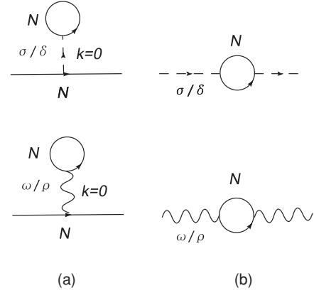
FIG. 1. Loop-diagram corrections to the self-energy of nucleons (a) and mesons (b) in nuclear medium, where N denotes nucleon and k is the four-momentum of the meson.
