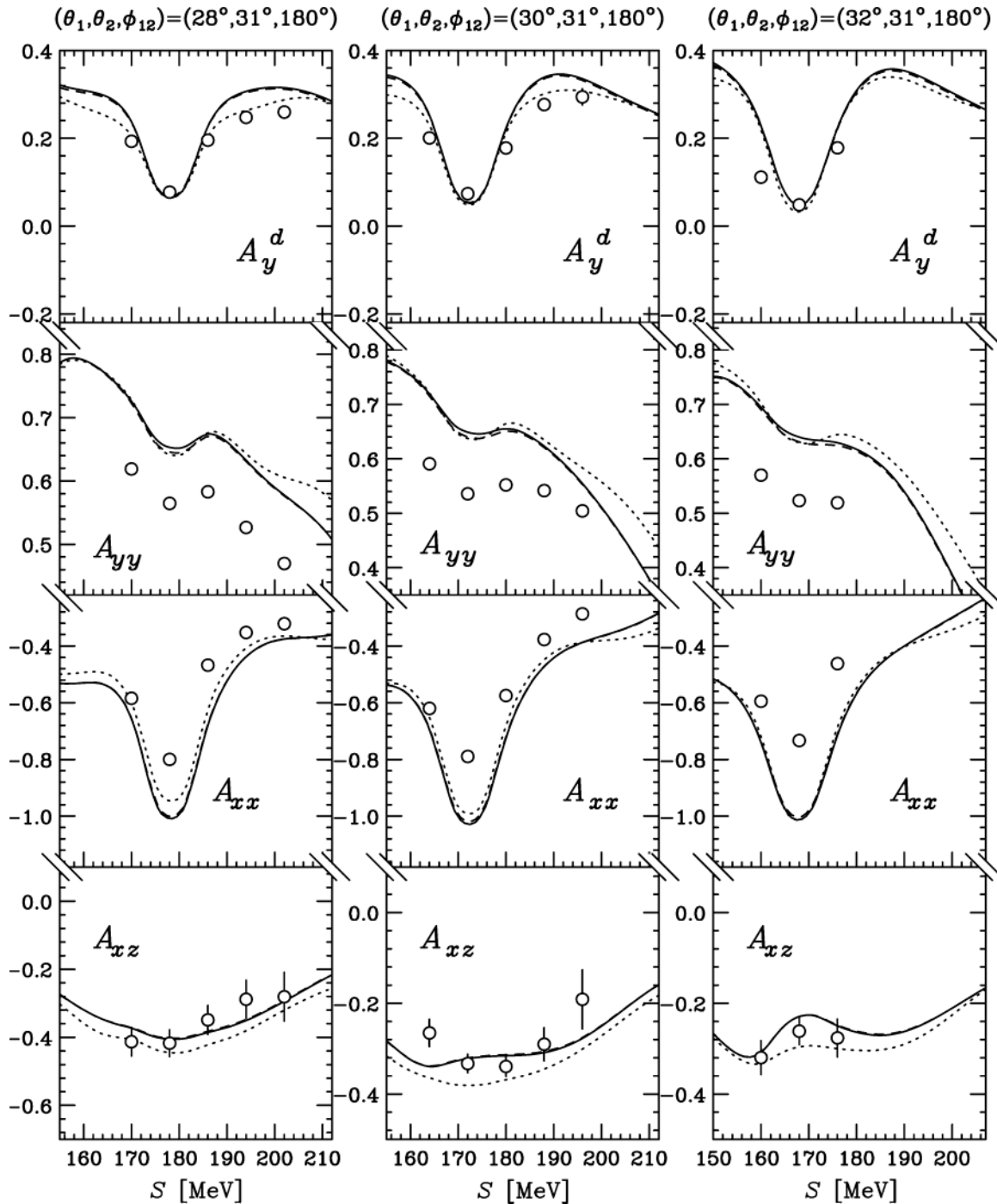
FIG. 12. Deuteron analyzing powers A_y^d , A_{xx} , A_{yy} , and A_{xz} for the complete breakup reaction {}^1\text{H}(\vec{d}, p_1 p_2)n at 135 MeV/nucleon and at the central positions of the detectors (\theta_1, \theta_2, \phi_{12}) as labeled. For the descriptions of the curves, see Fig. 11. All the theoretical predictions are point-geometry results averaged over the same energy bin \Delta S as the data (see text).
