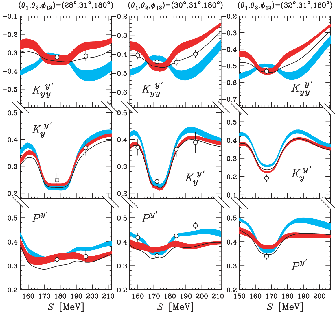
FIG. 7. (Color online) Polarization transfer coefficients K_{yy}^{y'} and K_y^{y'} and the induced polarization P^{y'} for the kinematically complete breakup reaction {}^1\text{H}(\vec{d}, \vec{p}_1 p_2)n at 135 MeV/nucleon at the central positions of the detectors ( \theta_1, \theta_2, \phi_{12} , as labeled at the top of each column) in the laboratory system. The shown S values are obtained with the nonrelativistic frame, and the experimental S values obtained with the relativistic frame are shifted by \delta S for each kinematical configuration (see text). The light shaded bands indicate the NN force predictions obtained with the AV18, CD-Bonn, Nijmegen I, and Nijmegen II potentials, and the dark shaded bands indicate the predictions when they are combined with the TM'(99) 3NF as described in the text. The solid curve is the AV18 + Urbana IX 3NF prediction. All the theoretical predictions are point-geometry results averaged over the same energy bin \Delta S as the data (see text).
