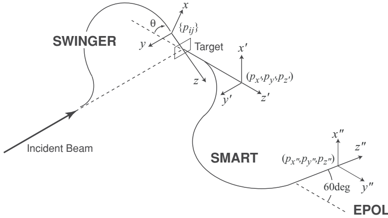
FIG. 6. Definition of the coordinate frame for the polarization observables at the SMART system. \{p_{ij}\} denotes the vector or tensor deuteron beam polarizations, p_i is the polarization of the scattered protons at the target position, and p_i'' is the polarization of the scattered protons at the second focal plane FP2.
