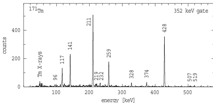
FIG. 2. Spectrum of \gamma rays in coincidence with the 352 keV transition in ^{171}\text{Tm} , with the additional requirement that the events occur between beam bursts. The labeled \gamma -ray transitions are included in the level scheme (Fig. 1).
