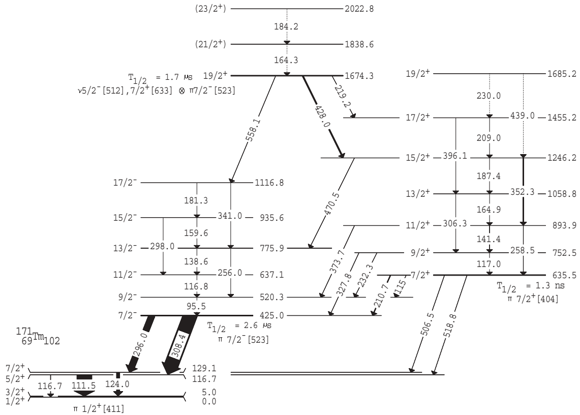
FIG. 1. Partial level scheme for ^{171}\text{Tm} , associated with the K^\pi = 19/2^+ isomer and its decay. The energies are those obtained in the present study. The 7/2^+ , 636 keV level and those fed from its decay, as well as the members of the 7/2^- band, were known from previous work [7,8].
