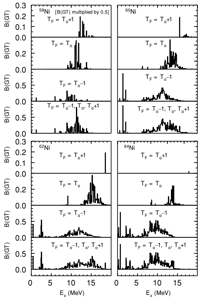
FIG. 4. B(\text{GT}) for ^{58,60,62,64}\text{Ni} to ^{58,60,62,64}\text{Cu} from the shell model calculations described in the text.
