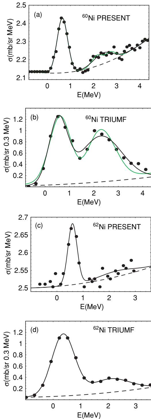
FIG. 5. (Color online) (a) Spectrum for ^{60}\text{Ni}(p, n)^{60}\text{Cu} ( T = 3 ) at 134.3 MeV, in the region of the T_o + 1 states. The black and gray (black and green on-line) curves are two- and three-Gaussian fits, respectively. (b) Spectrum for ^{60}\text{Ni}(n, p)^{60}\text{Co} at 198 MeV. The black and gray (black and green on-line) curves are two- and three-Gaussian fits, respectively. (c) Spectrum for ^{62}\text{Ni}(p, n)^{62}\text{Cu} ( T = 4 ) at 134.3 MeV, in the region of the T_o + 1 states. (d) Spectrum for ^{62}\text{Ni}(n, p)^{62}\text{Co} at 198 MeV. The 198 MeV data are from Ref. [4] and the 134.3 MeV data are from the present work. Spectra are fitted with a second order polynomial background and two or three Gaussian peaks. For details see the text.
