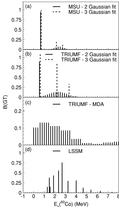
FIG. 6. Values of B(\text{GT}) for ^{60}\text{Ni} obtained from the present 134.3 MeV ( p, n ) data and the 198 MeV TRIUMF ( n, p ) data. (a) and (b) show the results of the fits to the ( p, n ) and the ( n, p ) cross sections as described in the text and shown in Fig. 5. (c) shows B(\text{GT}) from the multipole decomposition analysis (MDA) performed in Williams [4], and shown in their Fig. 12. The results from large scale shell model calculations [2] are shown in (d). For details see the text.
