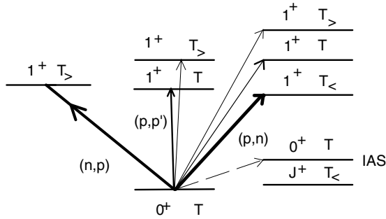
FIG. 1. Diagram of transitions via (p, n) , (n, p) , and (p, p') interactions. More intense transitions are shown by darker lines. With the exception of the transition to the isobaric analog state, those shown involve transfer of total angular momentum, spin, and isospin \Delta J = \Delta S = \Delta T = 1 . States labeled with the same quantum numbers are isobaric analogs. The symbols T_> , T , and T_< stand for T_o + 1 , T_o , and T_o - 1 . We are concerned here with the relatively weak (p, n) transitions to the 1^+ , T_> states.
