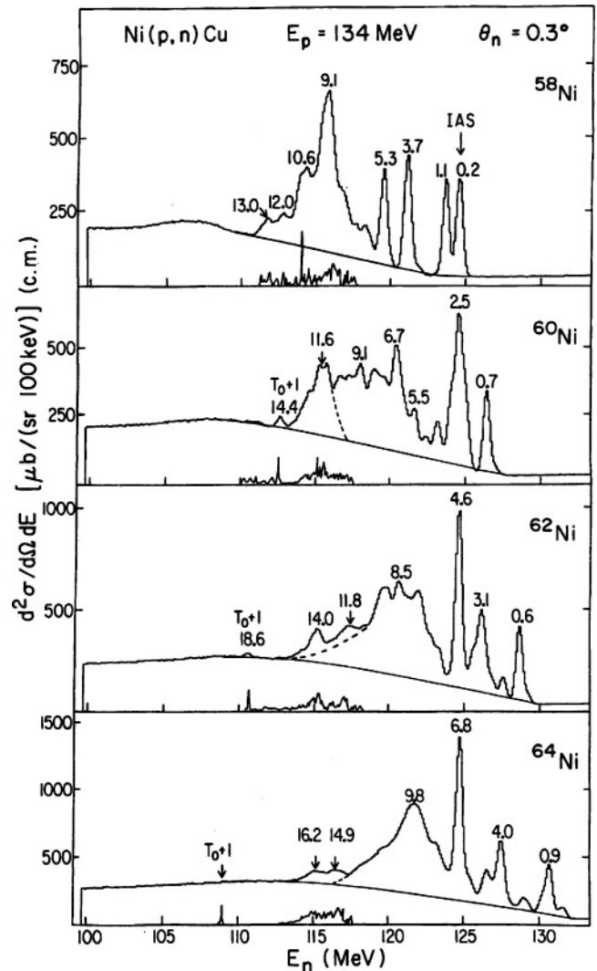
FIG. 2. Spectra for 58,60,62,64 Ni (p, n) reactions at 134.4 MeV. There are about 10 4 counts per channel for a channel width of about 150(115) keV for the 60 Ni( 62 Ni) spectrum in the region of the T_o+1 peaks. This is sufficient to observe the weak T_o + 1 states as described in the text. The numbers above the peaks in the spectra are excitation energies. Spectra observed in (p, p') reactions [18] on the target nuclei are plotted on the energy axis. The sharp peak toward the left of each (p, p') spectrum is the lowest-lying T_o + 1 state.
