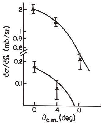
FIG. 3. Angular distributions for the T_o + 1 excitations in ^{60}\text{Ni} (upper points) and ^{62}\text{Ni} (lower points); the points are the cross sections above the smooth background for the lowest lying T_o + 1 peak in Fig. 2. The ^{60}\text{Ni} cross sections have been multiplied by 10 for display purposes. The curves are the DWBA calculations described in the text.
