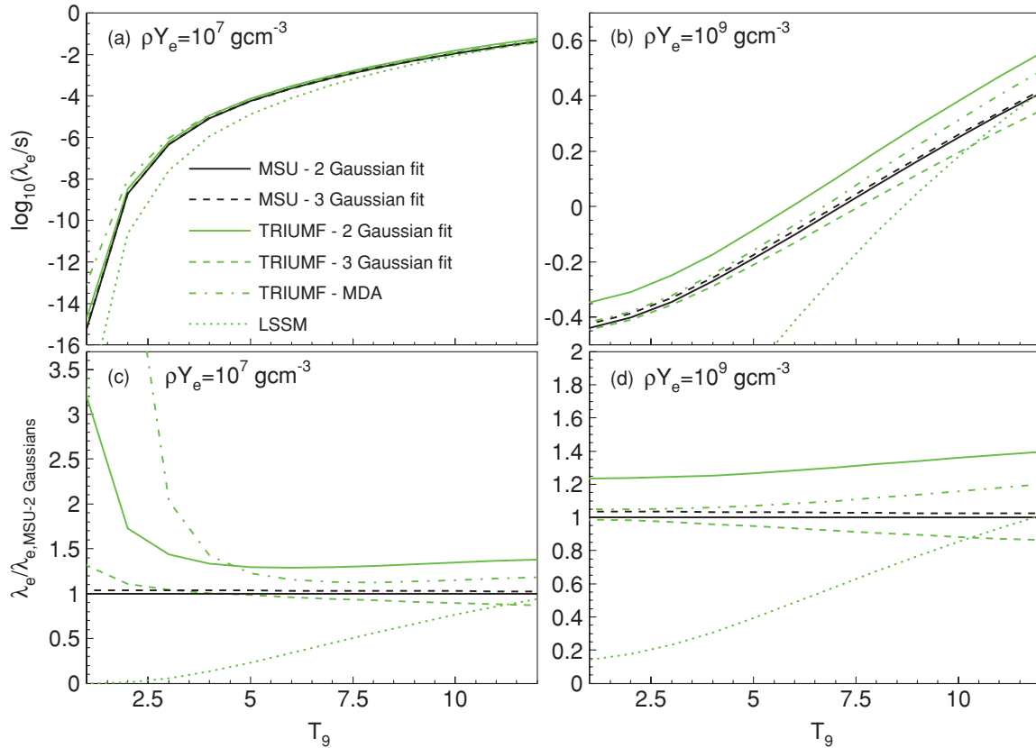
FIG. 7. (Color online) Reaction rates obtained from the B(\text{GT}) of Fig. 6. The upper two panels show the absolute rates and the lower two panels the results compared to those for the 134.3 MeV (p, n) data. For details see the text.
